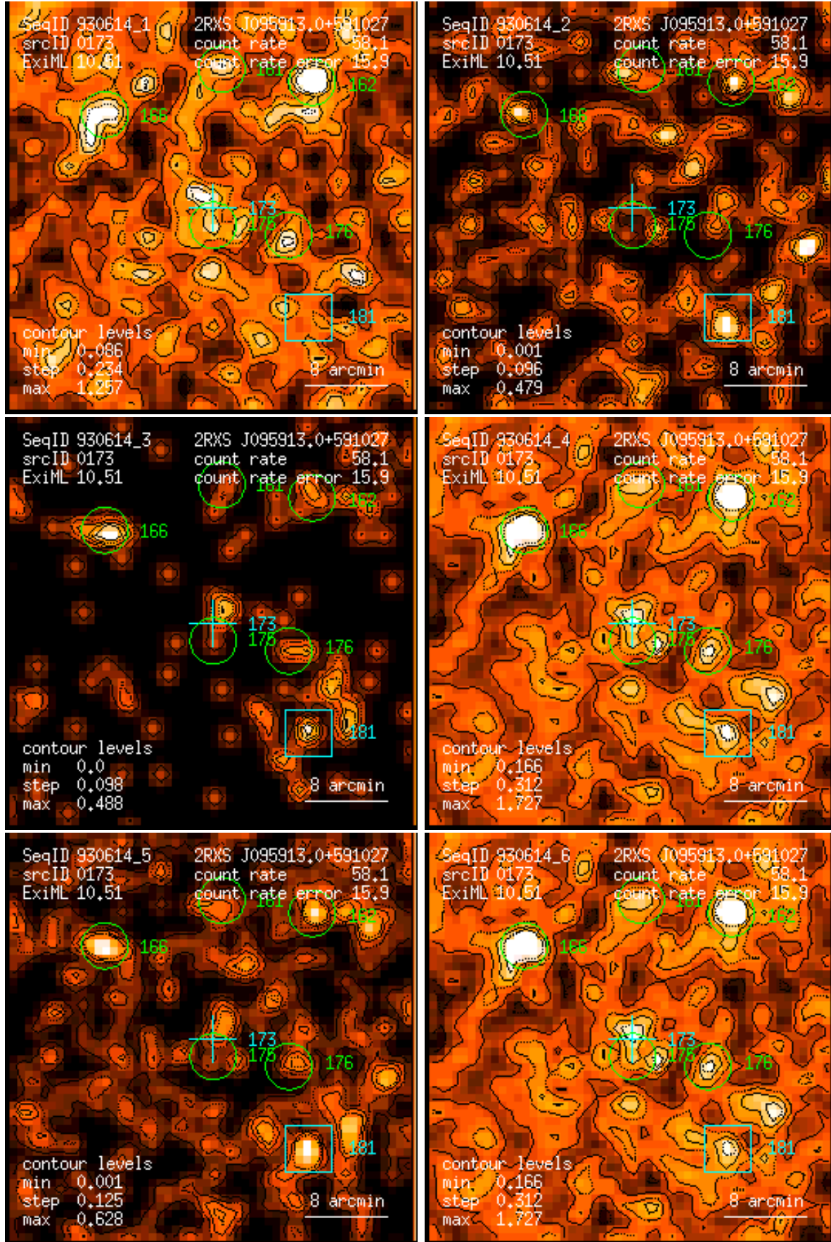
Figure 173: RASS 930614: detection 0173: band rate images, Gaussian filter: (1) PSPC channels 11 – 41, (2) 52 – 90, (3) 91 – 201, (4) 11 – 235, (5) 52 – 201, (6) 11 – 201. Broad band rates in counts/ks. Band rate contour levels in counts/ks/arcmin 2 .
