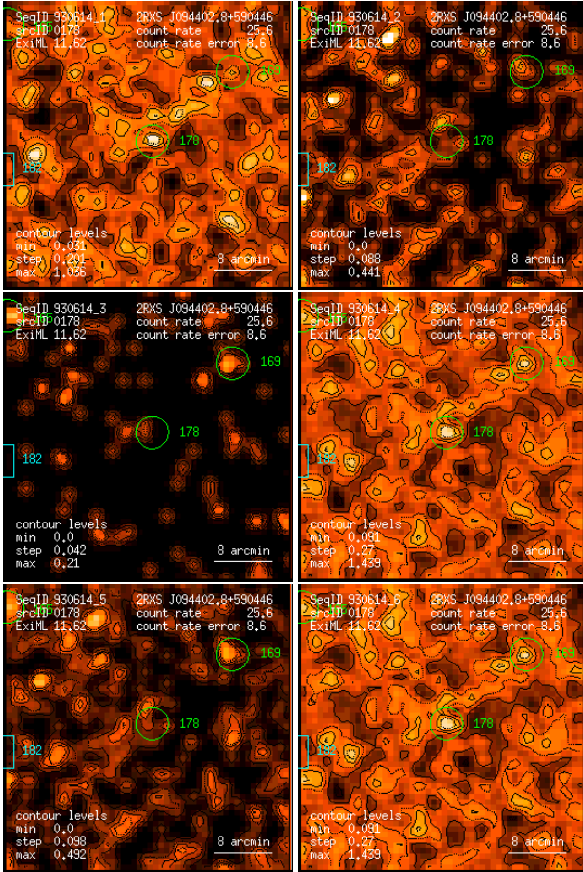
Figure 178: RASS 930614: detection 0178: band rate images, Gaussian filter: (1) PSPC channels 11 – 41, (2) 52 – 90, (3) 91 – 201, (4) 11 – 235, (5) 52 – 201, (6) 11 – 201. Broad band rates in counts/ks. Band rate contour levels in counts/ks/arcmin 2 .
