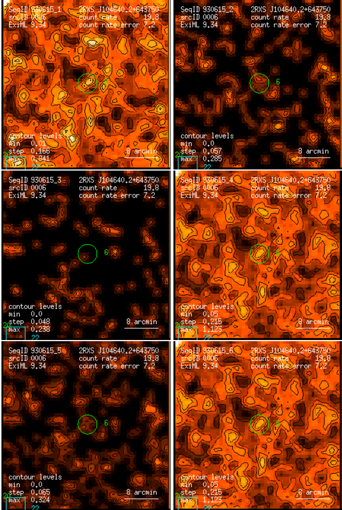
Figure 6: RASS 930615: detection 0006: band rate images, Gaussian filter: (1) PSPC channels 11 – 41, (2) 52 – 90, (3) 91 – 201, (4) 11 – 235, (5) 52 – 201, (6) 11 – 201. Broad band rates in counts/ks. Band rate contour levels in counts/ks/arcmin 2 .
