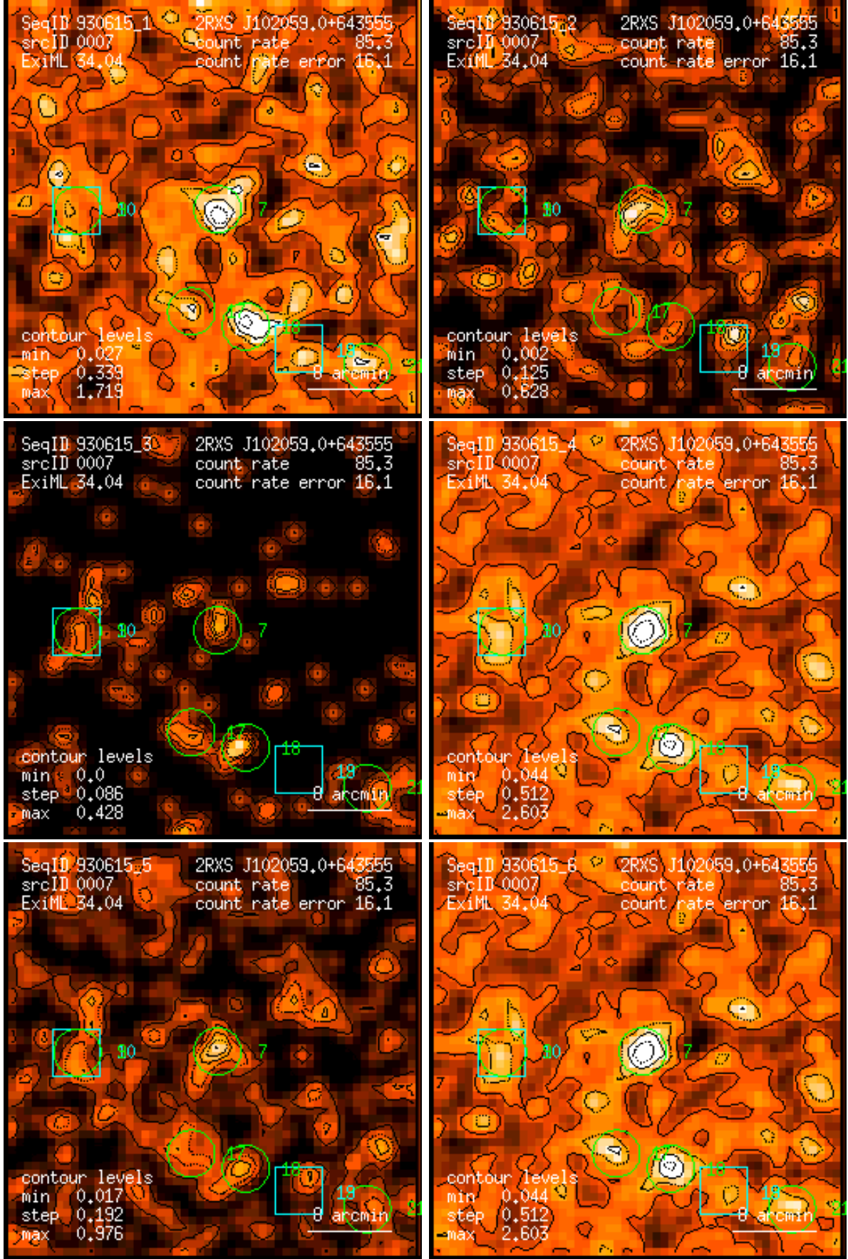
Figure 7: RASS 930615: detection 0007: band rate images, Gaussian filter: (1) PSPC channels 11 – 41, (2) 52 – 90, (3) 91 – 201, (4) 11 – 235, (5) 52 – 201, (6) 11 – 201. Broad band rates in counts/ks. Band rate contour levels in counts/ks/arcmin 2 .
