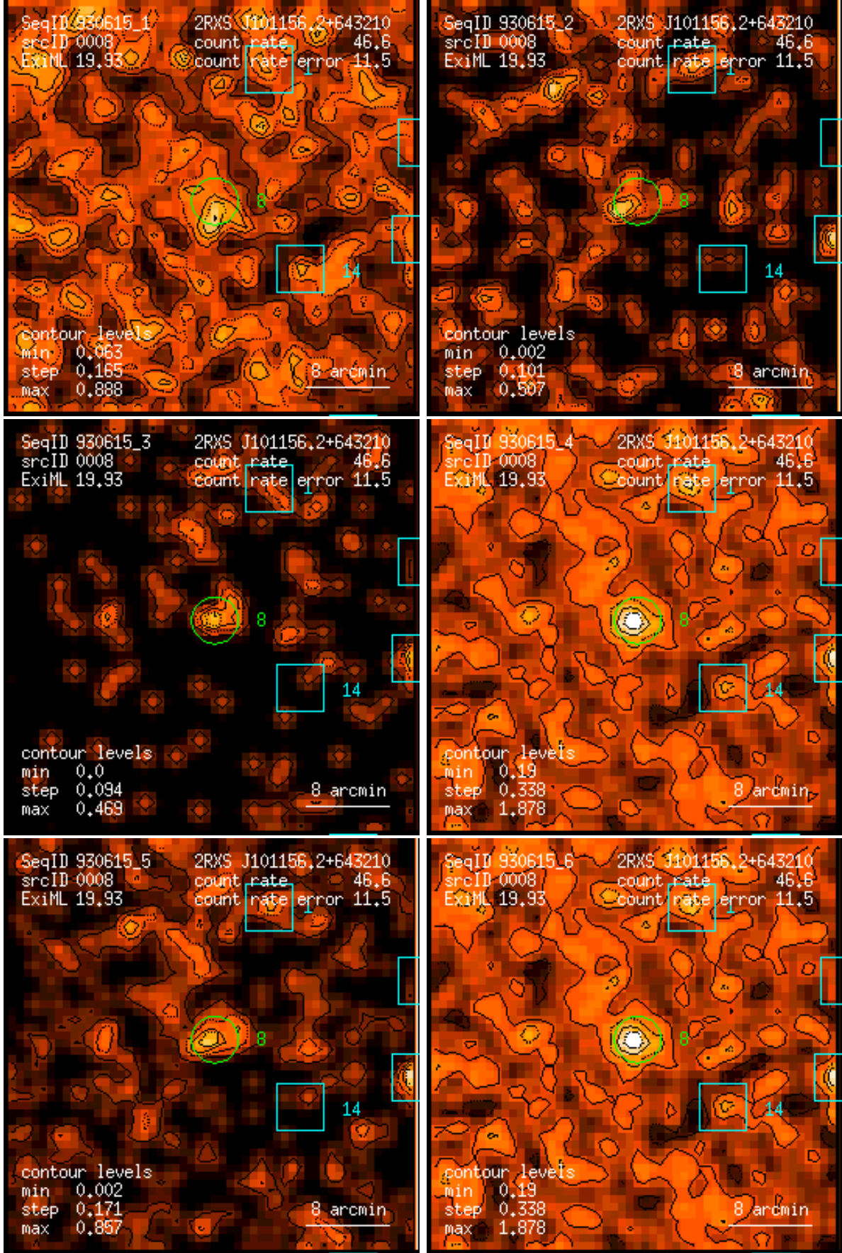
Figure 8: RASS 930615: detection 0008: band rate images, Gaussian filter: (1) PSPC channels 11 – 41, (2) 52 – 90, (3) 91 – 201, (4) 11 – 235, (5) 52 – 201, (6) 11 – 201. Broad band rates in counts/ks. Band rate contour levels in counts/ks/arcmin 2 .
