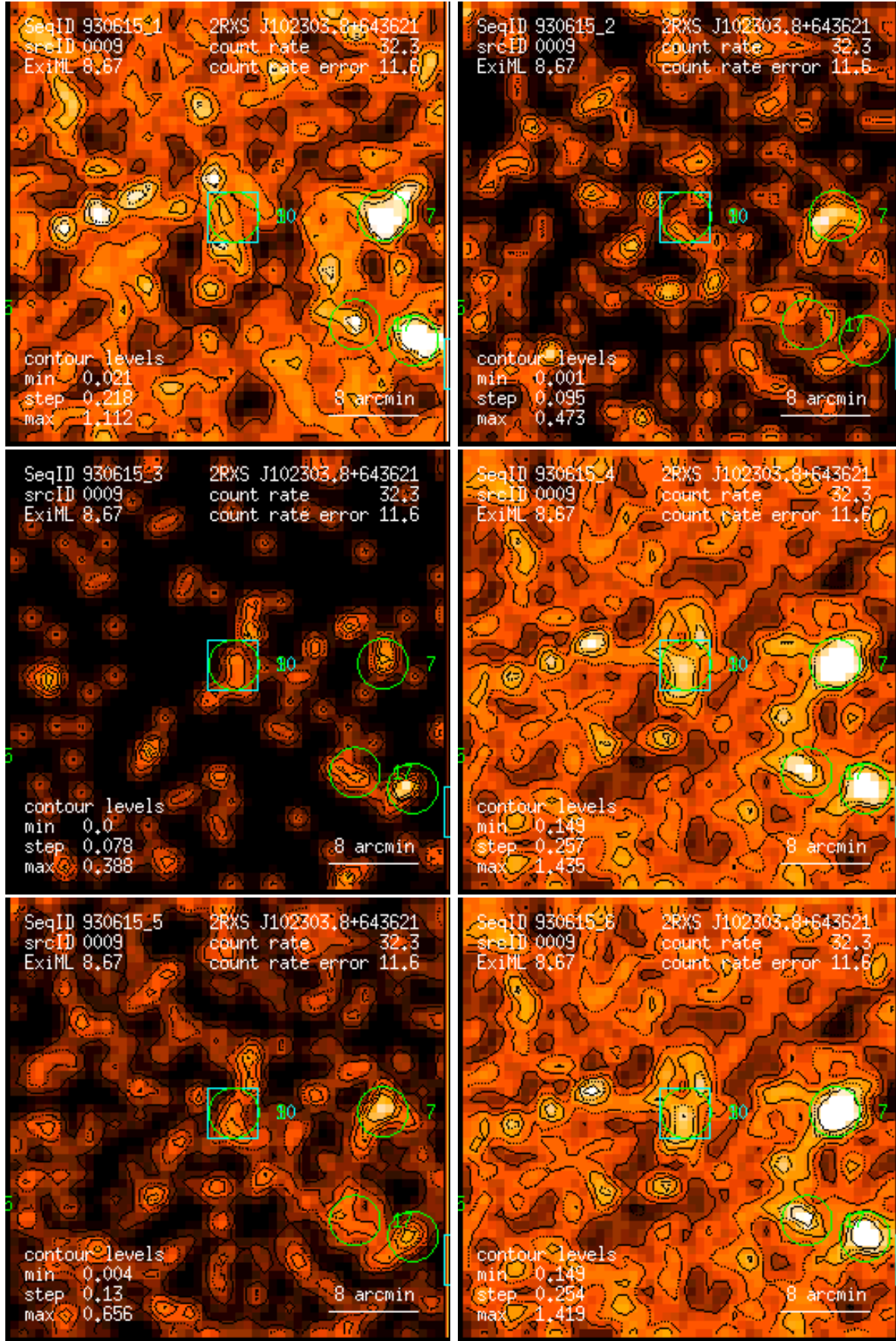
Figure 9: RASS 930615: detection 0009: band rate images, Gaussian filter: (1) PSPC channels 11 – 41, (2) 52 – 90, (3) 91 – 201, (4) 11 – 235, (5) 52 – 201, (6) 11 – 201. Broad band rates in counts/ks. Band rate contour levels in counts/ks/arcmin 2 .
