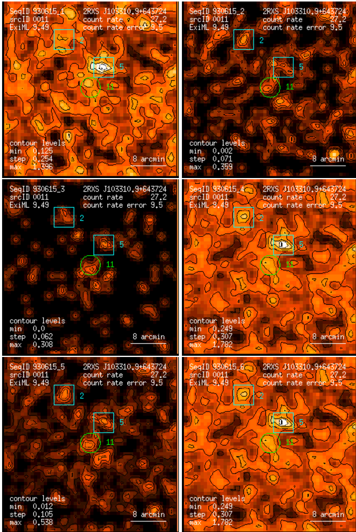
Figure 11: RASS 930615: detection 0011: band rate images, Gaussian filter: (1) PSPC channels 11 – 41, (2) 52 – 90, (3) 91 – 201, (4) 11 – 235, (5) 52 – 201, (6) 11 – 201. Broad band rates in counts/ks. Band rate contour levels in counts/ks/arcmin 2 .
