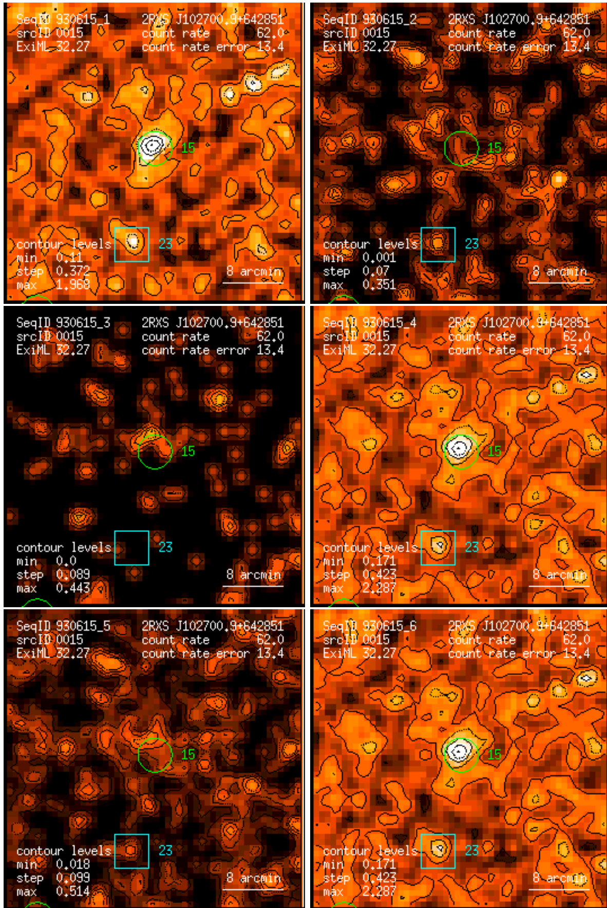
Figure 15: RASS 930615: detection 0015: band rate images, Gaussian filter: (1) PSPC channels 11 – 41, (2) 52 – 90, (3) 91 – 201, (4) 11 – 235, (5) 52 – 201, (6) 11 – 201. Broad band rates in counts/ks. Band rate contour levels in counts/ks/arcmin 2 .
