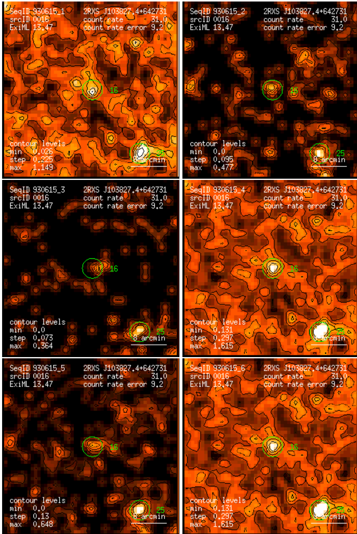
Figure 16: RASS 930615: detection 0016: band rate images, Gaussian filter: (1) PSPC channels 11 – 41, (2) 52 – 90, (3) 91 – 201, (4) 11 – 235, (5) 52 – 201, (6) 11 – 201. Broad band rates in counts/ks. Band rate contour levels in counts/ks/arcmin 2 .
