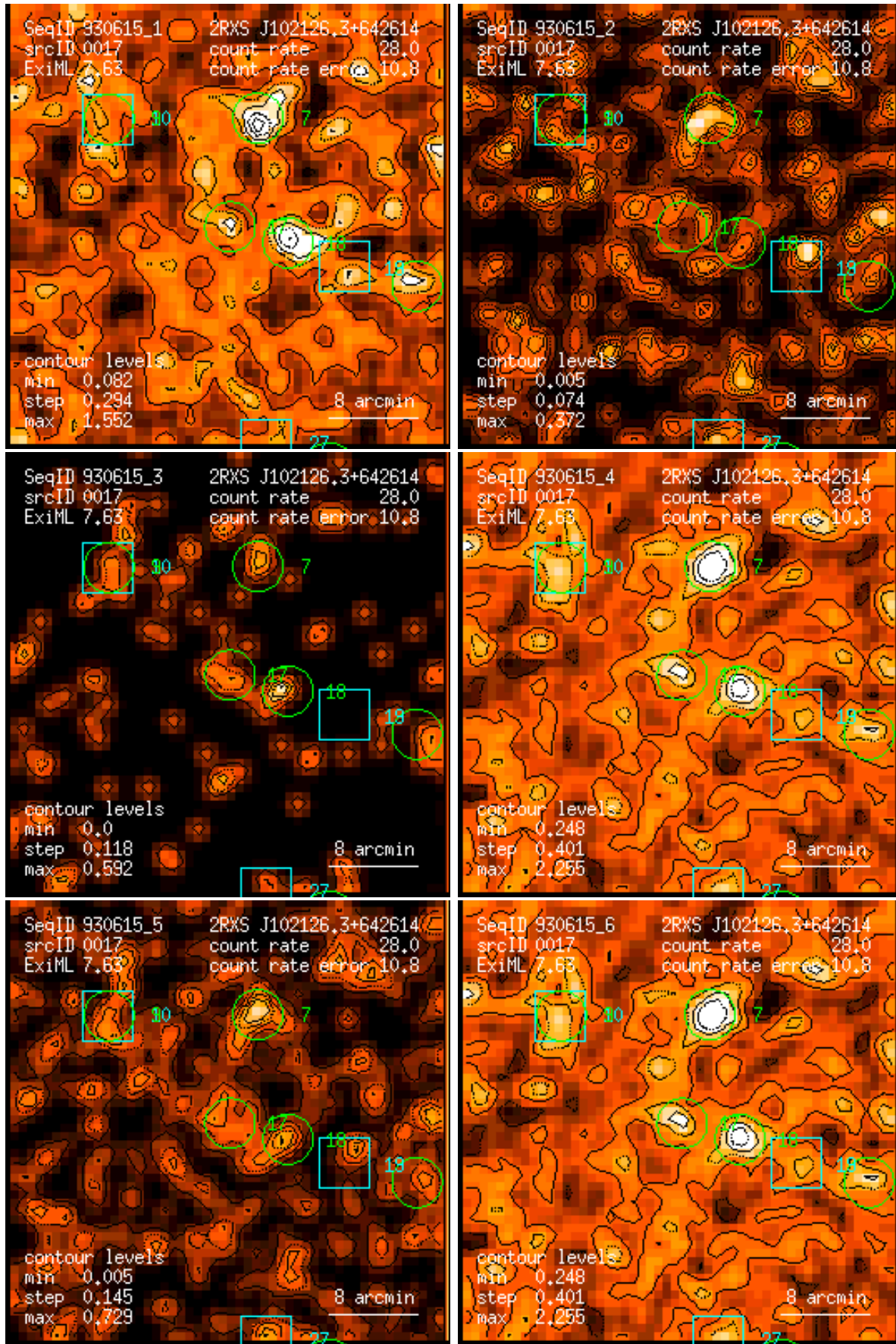
Figure 17: RASS 930615: detection 0017: band rate images, Gaussian filter: (1) PSPC channels 11 – 41, (2) 52 – 90, (3) 91 – 201, (4) 11 – 235, (5) 52 – 201, (6) 11 – 201. Broad band rates in counts/ks. Band rate contour levels in counts/ks/arcmin 2 .
