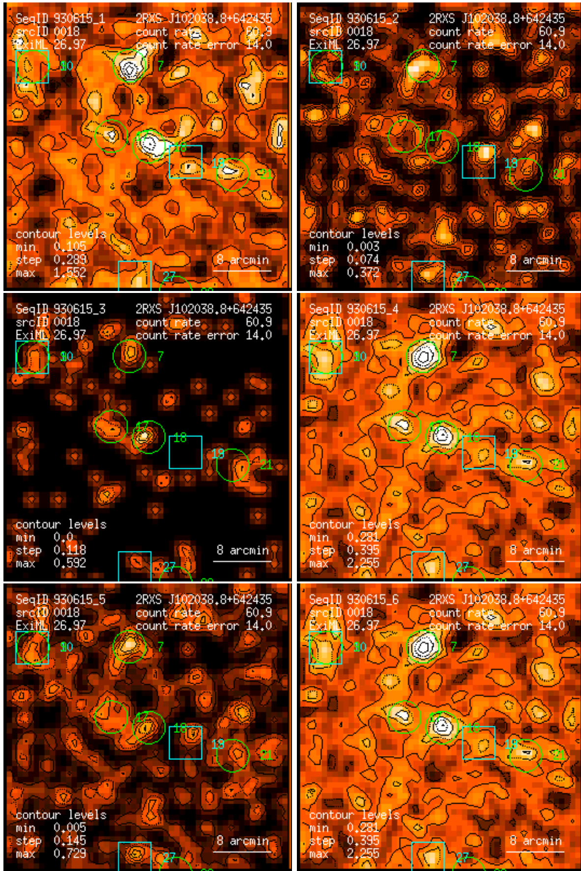
Figure 18: RASS 930615: detection 0018: band rate images, Gaussian filter: (1) PSPC channels 11 – 41, (2) 52 – 90, (3) 91 – 201, (4) 11 – 235, (5) 52 – 201, (6) 11 – 201. Broad band rates in counts/ks. Band rate contour levels in counts/ks/arcmin 2 .
