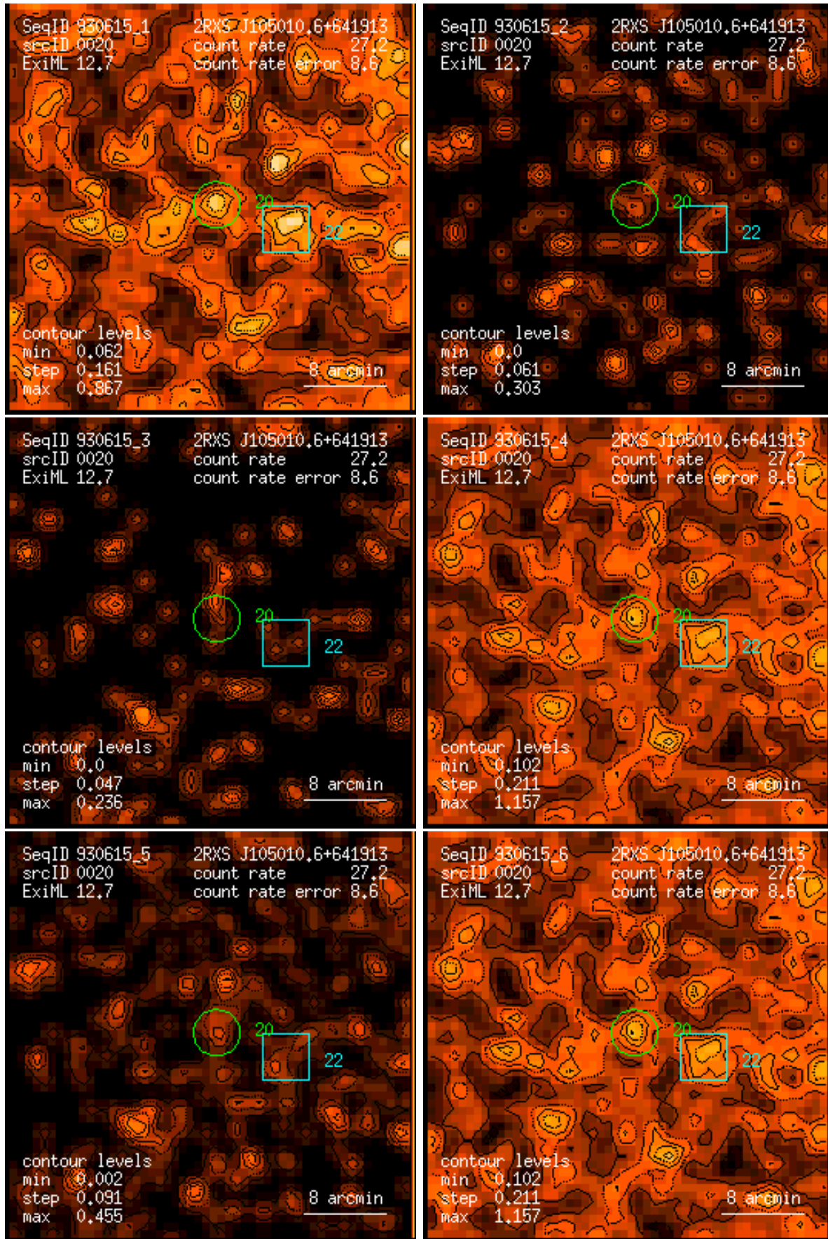
Figure 20: RASS 930615: detection 0020: band rate images, Gaussian filter: (1) PSPC channels 11 – 41, (2) 52 – 90, (3) 91 – 201, (4) 11 – 235, (5) 52 – 201, (6) 11 – 201. Broad band rates in counts/ks. Band rate contour levels in counts/ks/arcmin 2 .
