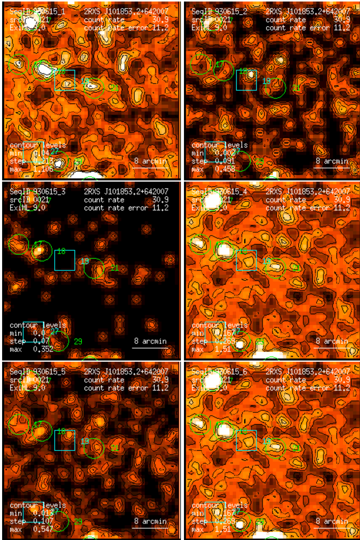
Figure 21: RASS 930615: detection 0021: band rate images, Gaussian filter: (1) PSPC channels 11 – 41, (2) 52 – 90, (3) 91 – 201, (4) 11 – 235, (5) 52 – 201, (6) 11 – 201. Broad band rates in counts/ks. Band rate contour levels in counts/ks/arcmin 2 .
