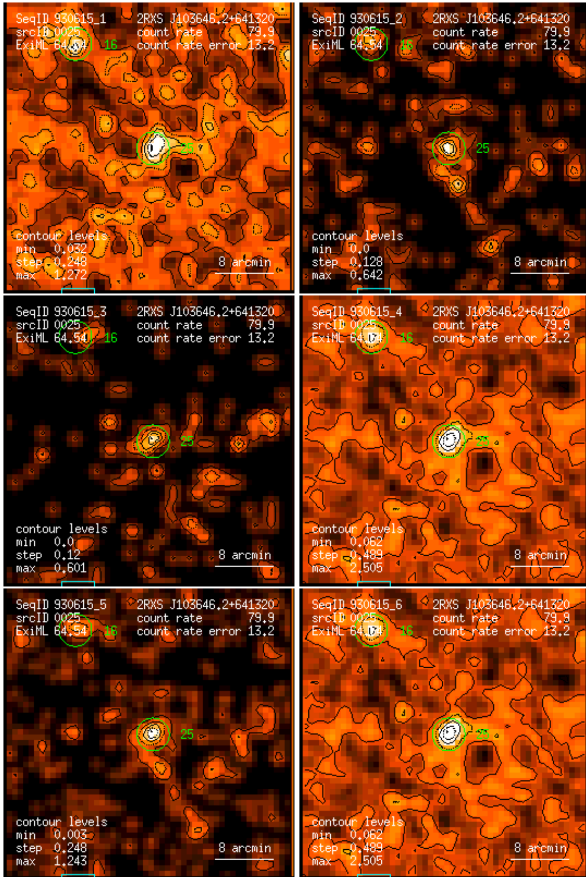
Figure 25: RASS 930615: detection 0025: band rate images, Gaussian filter: (1) PSPC channels 11 – 41, (2) 52 – 90, (3) 91 – 201, (4) 11 – 235, (5) 52 – 201, (6) 11 – 201. Broad band rates in counts/ks. Band rate contour levels in counts/ks/arcmin 2 .
