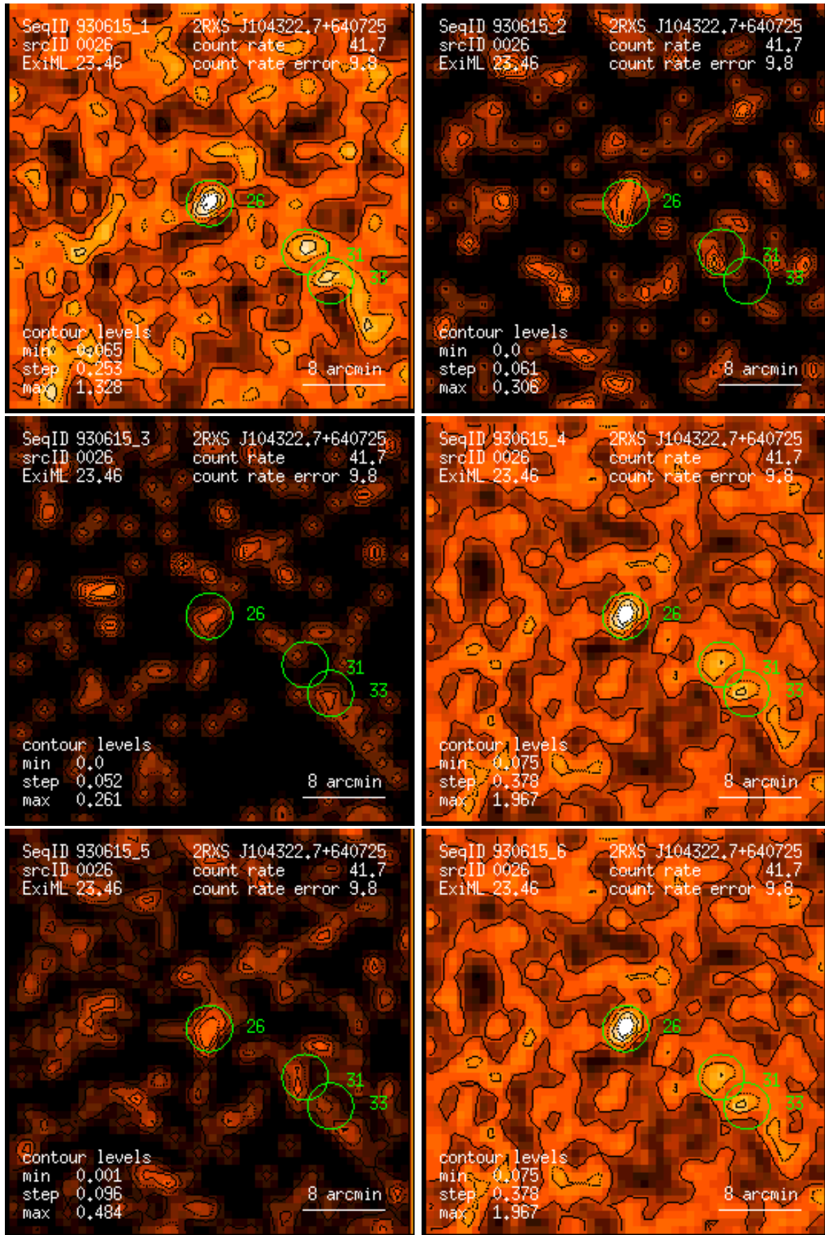
Figure 26: RASS 930615: detection 0026: band rate images, Gaussian filter: (1) PSPC channels 11 – 41, (2) 52 – 90, (3) 91 – 201, (4) 11 – 235, (5) 52 – 201, (6) 11 – 201. Broad band rates in counts/ks. Band rate contour levels in counts/ks/arcmin 2 .
