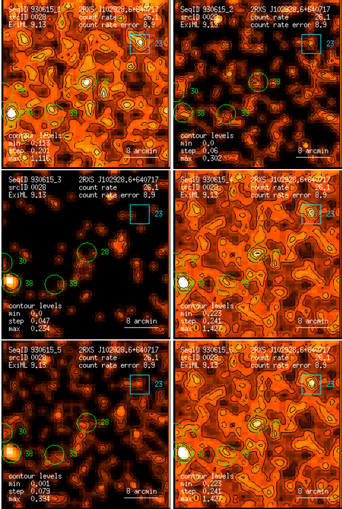
Figure 28: RASS 930615: detection 0028: band rate images, Gaussian filter: (1) PSPC channels 11 – 41, (2) 52 – 90, (3) 91 – 201, (4) 11 – 235, (5) 52 – 201, (6) 11 – 201. Broad band rates in counts/ks. Band rate contour levels in counts/ks/arcmin 2 .
