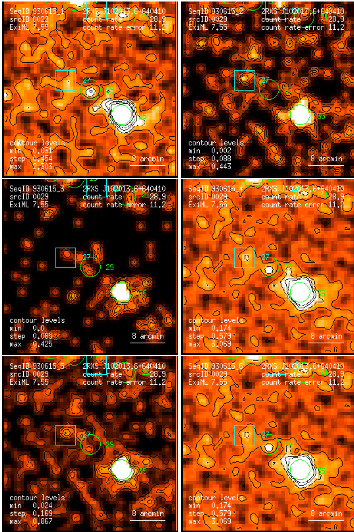
Figure 29: RASS 930615: detection 0029: band rate images, Gaussian filter: (1) PSPC channels 11 – 41, (2) 52 – 90, (3) 91 – 201, (4) 11 – 235, (5) 52 – 201, (6) 11 – 201. Broad band rates in counts/ks. Band rate contour levels in counts/ks/arcmin 2 .
