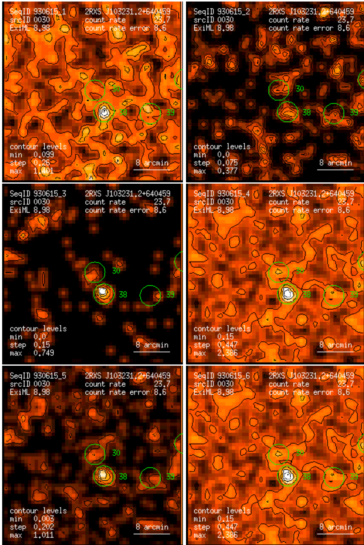
Figure 30: RASS 930615: detection 0030: band rate images, Gaussian filter: (1) PSPC channels 11 – 41, (2) 52 – 90, (3) 91 – 201, (4) 11 – 235, (5) 52 – 201, (6) 11 – 201. Broad band rates in counts/ks. Band rate contour levels in counts/ks/arcmin 2 .
