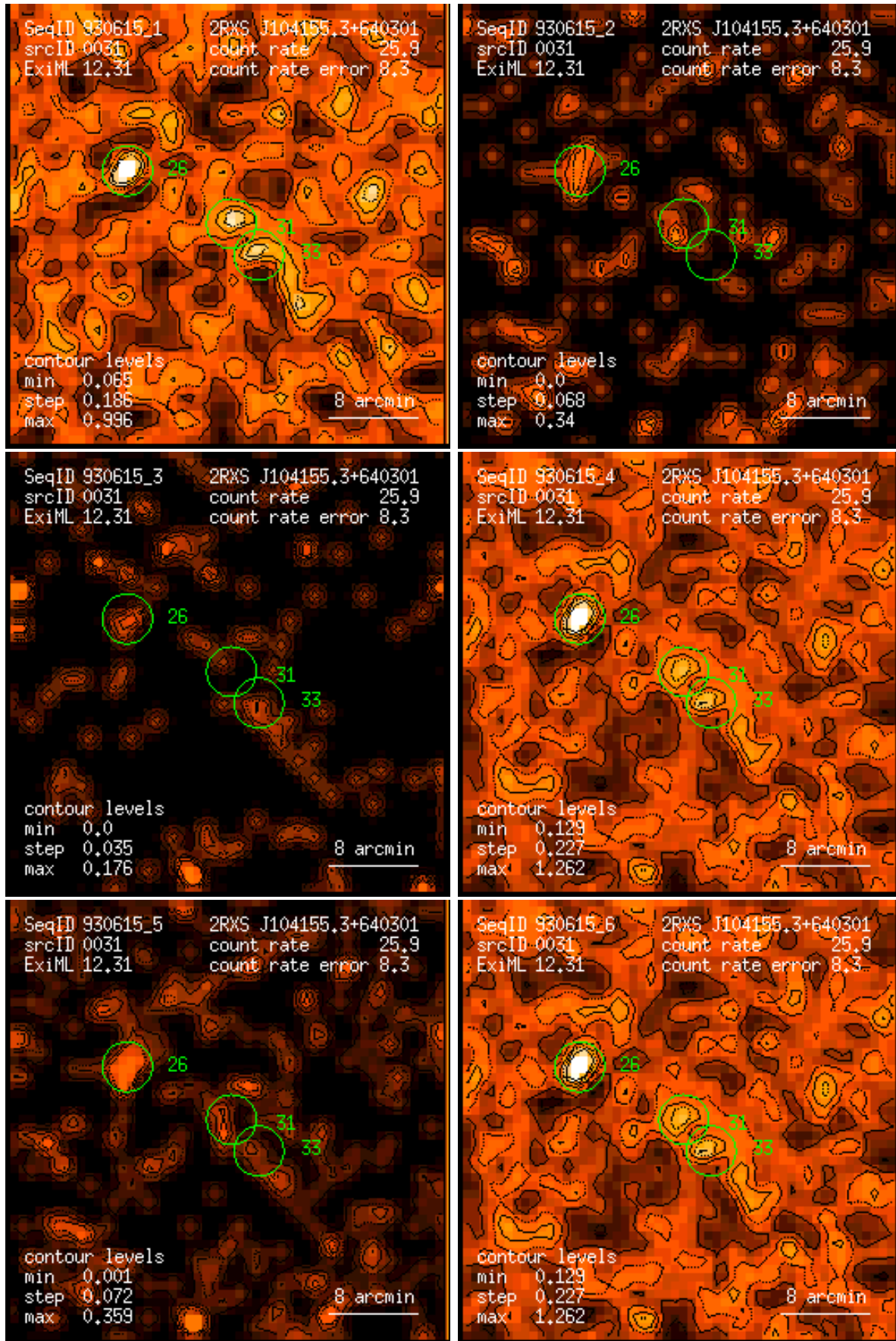
Figure 31: RASS 930615: detection 0031: band rate images, Gaussian filter: (1) PSPC channels 11 – 41, (2) 52 – 90, (3) 91 – 201, (4) 11 – 235, (5) 52 – 201, (6) 11 – 201. Broad band rates in counts/ks. Band rate contour levels in counts/ks/arcmin 2 .
