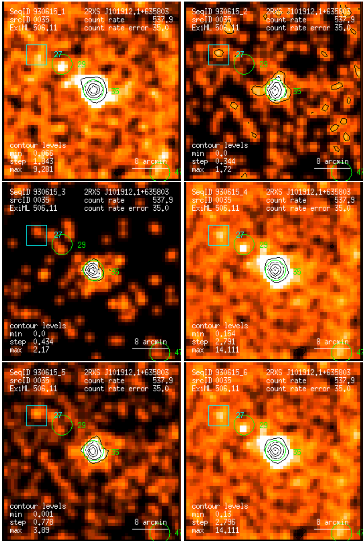
Figure 35: RASS 930615: detection 0035: band rate images, Gaussian filter: (1) PSPC channels 11 – 41, (2) 52 – 90, (3) 91 – 201, (4) 11 – 235, (5) 52 – 201, (6) 11 – 201. Broad band rates in counts/ks. Band rate contour levels in counts/ks/arcmin 2 .
