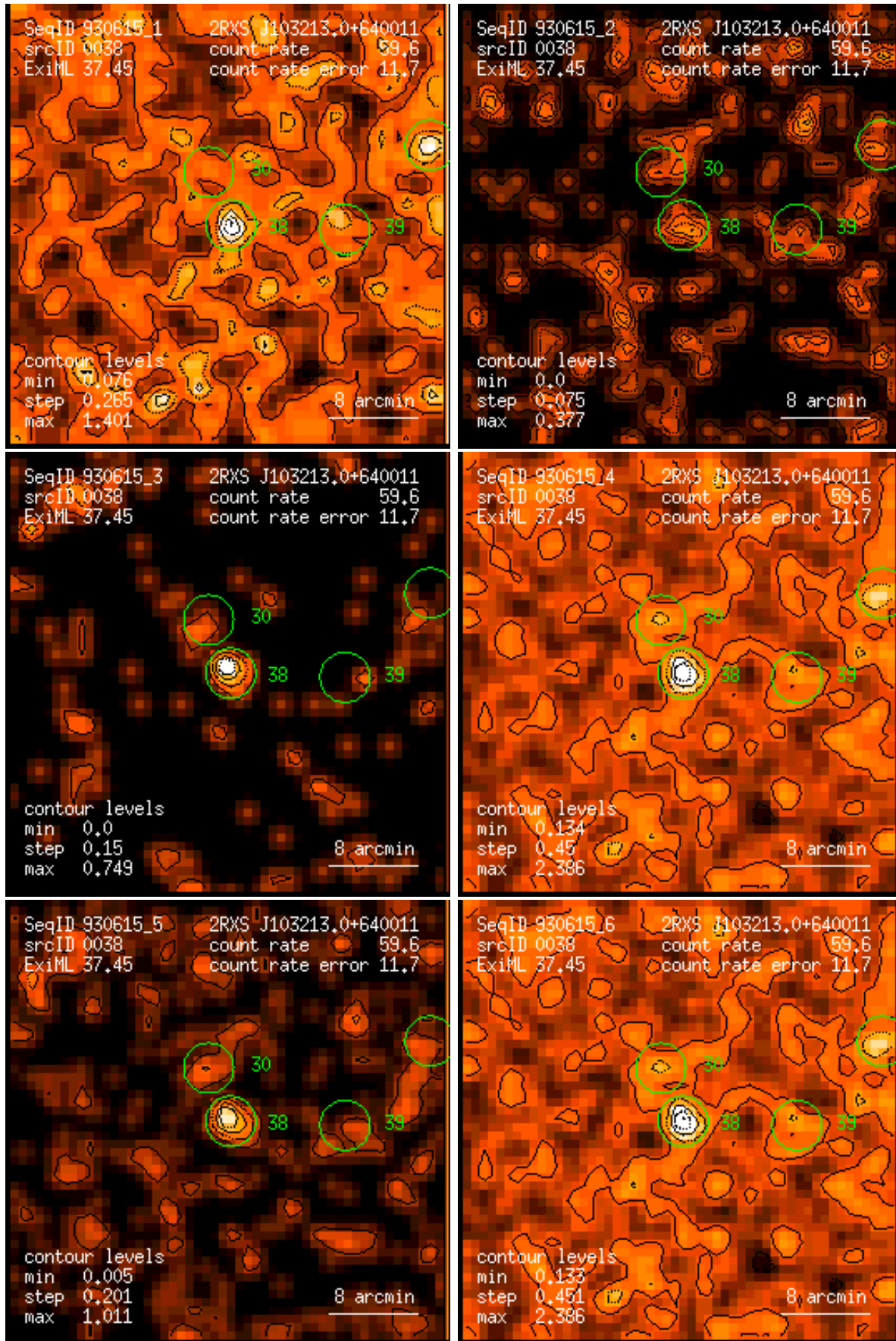
Figure 38: RASS 930615: detection 0038: band rate images, Gaussian filter: (1) PSPC channels 11 – 41, (2) 52 – 90, (3) 91 – 201, (4) 11 – 235, (5) 52 – 201, (6) 11 – 201. Broad band rates in counts/ks. Band rate contour levels in counts/ks/arcmin 2 .
