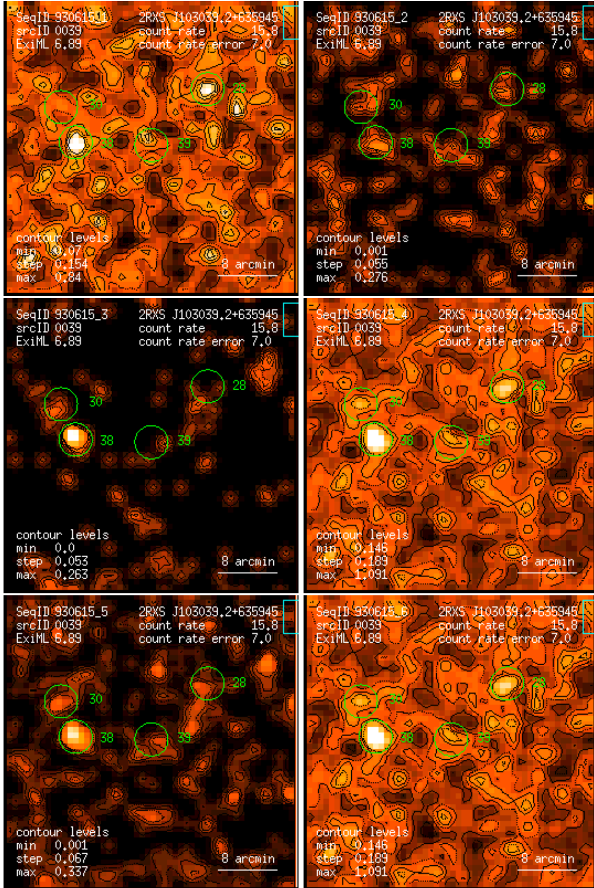
Figure 39: RASS 930615: detection 0039: band rate images, Gaussian filter: (1) PSPC channels 11 – 41, (2) 52 – 90, (3) 91 – 201, (4) 11 – 235, (5) 52 – 201, (6) 11 – 201. Broad band rates in counts/ks. Band rate contour levels in counts/ks/arcmin 2 .
