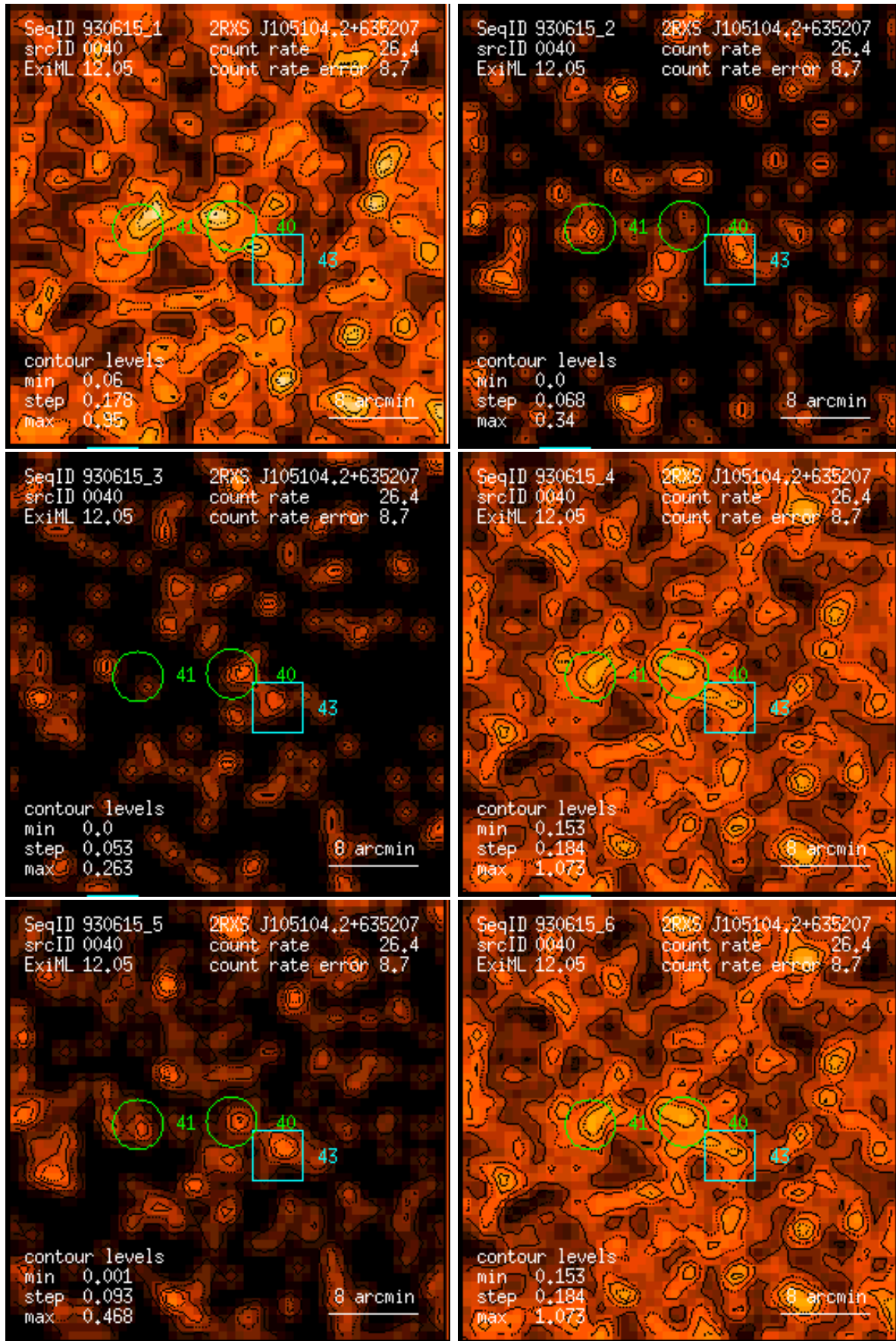
Figure 40: RASS 930615: detection 0040: band rate images, Gaussian filter: (1) PSPC channels 11 – 41, (2) 52 – 90, (3) 91 – 201, (4) 11 – 235, (5) 52 – 201, (6) 11 – 201. Broad band rates in counts/ks. Band rate contour levels in counts/ks/arcmin 2 .
