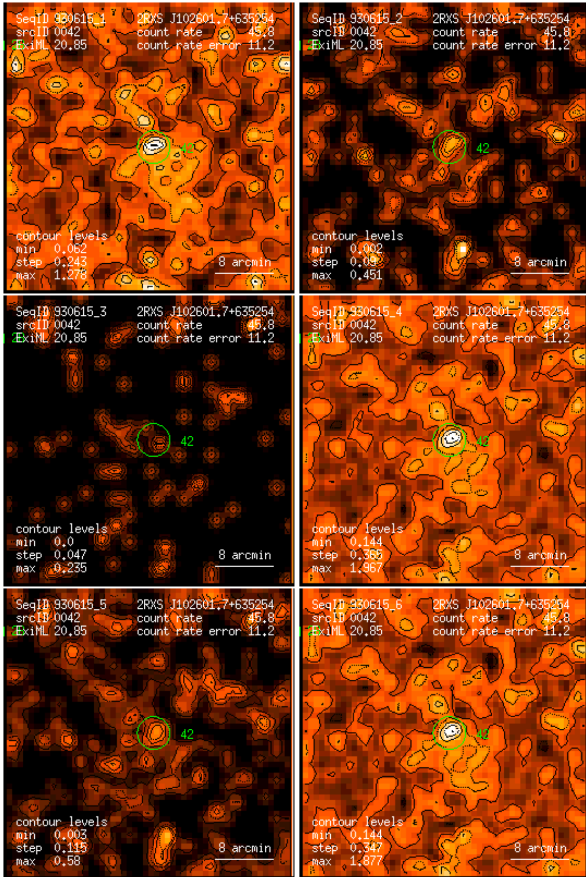
Figure 42: RASS 930615: detection 0042: band rate images, Gaussian filter: (1) PSPC channels 11 – 41, (2) 52 – 90, (3) 91 – 201, (4) 11 – 235, (5) 52 – 201, (6) 11 – 201. Broad band rates in counts/ks. Band rate contour levels in counts/ks/arcmin 2 .
