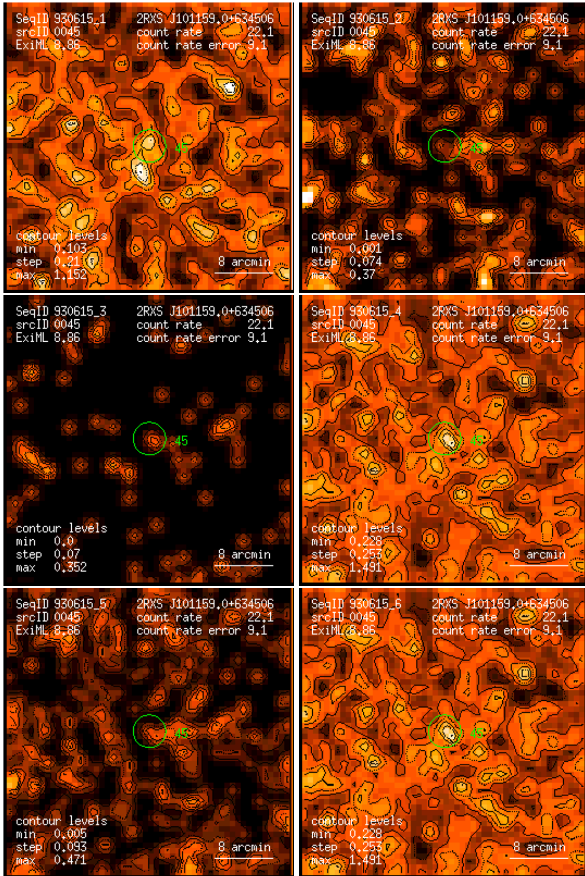
Figure 45: RASS 930615: detection 0045: band rate images, Gaussian filter: (1) PSPC channels 11 – 41, (2) 52 – 90, (3) 91 – 201, (4) 11 – 235, (5) 52 – 201, (6) 11 – 201. Broad band rates in counts/ks. Band rate contour levels in counts/ks/arcmin 2 .
