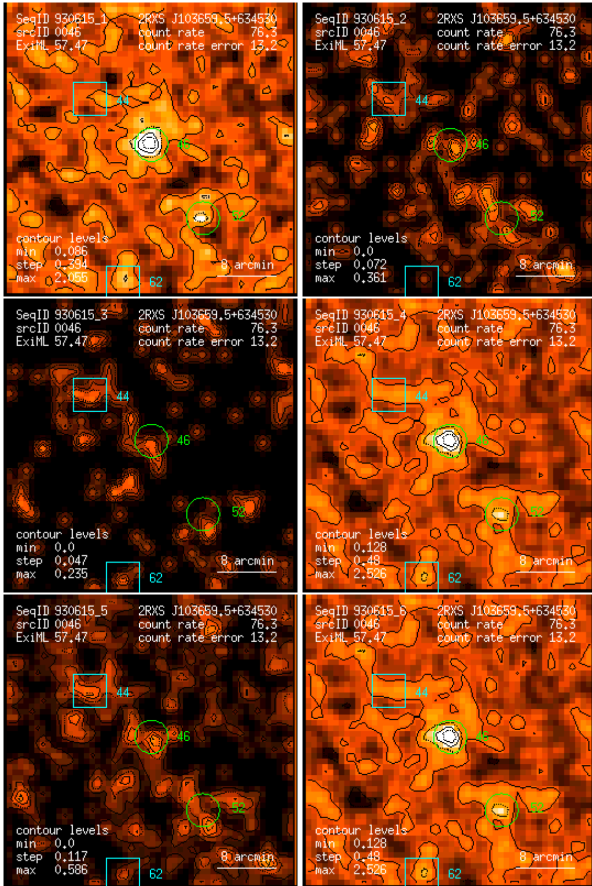
Figure 46: RASS 930615: detection 0046: band rate images, Gaussian filter: (1) PSPC channels 11 – 41, (2) 52 – 90, (3) 91 – 201, (4) 11 – 235, (5) 52 – 201, (6) 11 – 201. Broad band rates in counts/ks. Band rate contour levels in counts/ks/arcmin 2 .
