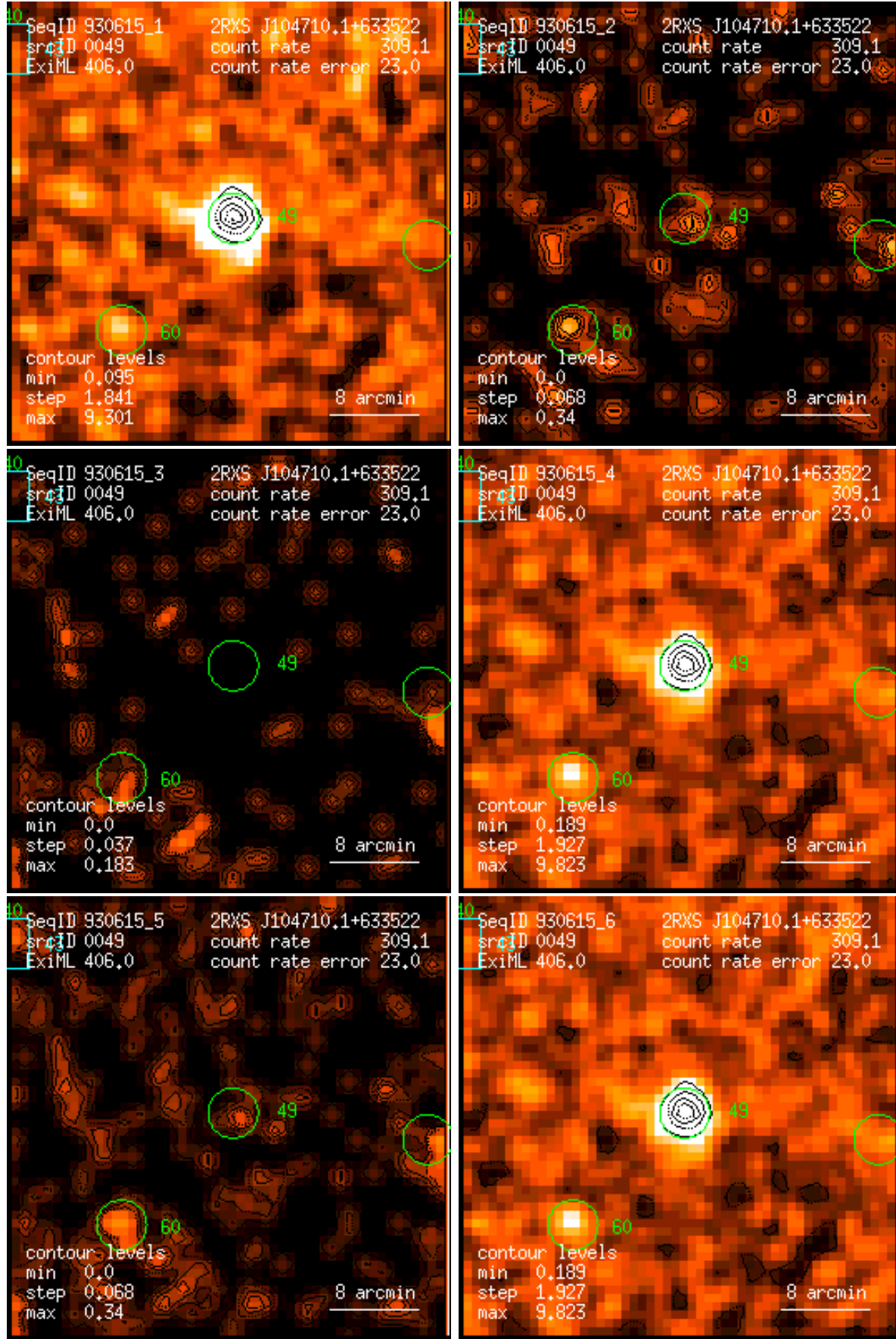
Figure 49: RASS 930615: detection 0049: band rate images, Gaussian filter: (1) PSPC channels 11 – 41, (2) 52 – 90, (3) 91 – 201, (4) 11 – 235, (5) 52 – 201, (6) 11 – 201. Broad band rates in counts/ks. Band rate contour levels in counts/ks/arcmin 2 .
