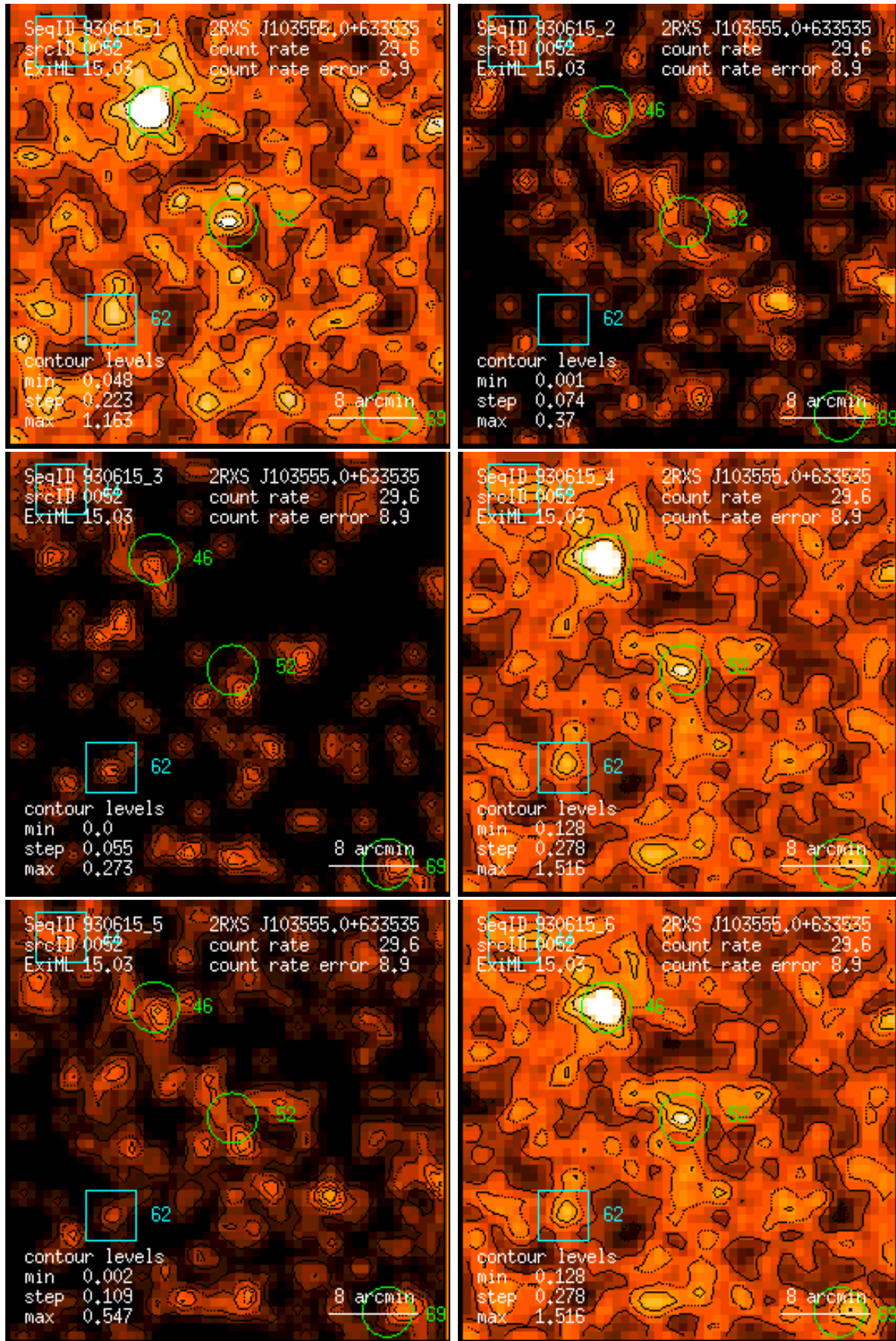
Figure 52: RASS 930615: detection 0052: band rate images, Gaussian filter: (1) PSPC channels 11 – 41, (2) 52 – 90, (3) 91 – 201, (4) 11 – 235, (5) 52 – 201, (6) 11 – 201. Broad band rates in counts/ks. Band rate contour levels in counts/ks/arcmin 2 .
