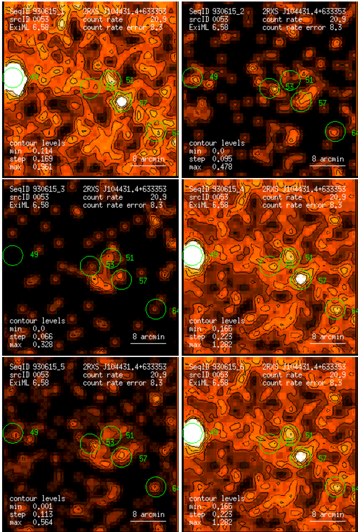
Figure 53: RASS 930615: detection 0053: band rate images, Gaussian filter: (1) PSPC channels 11 – 41, (2) 52 – 90, (3) 91 – 201, (4) 11 – 235, (5) 52 – 201, (6) 11 – 201. Broad band rates in counts/ks. Band rate contour levels in counts/ks/arcmin 2 .
