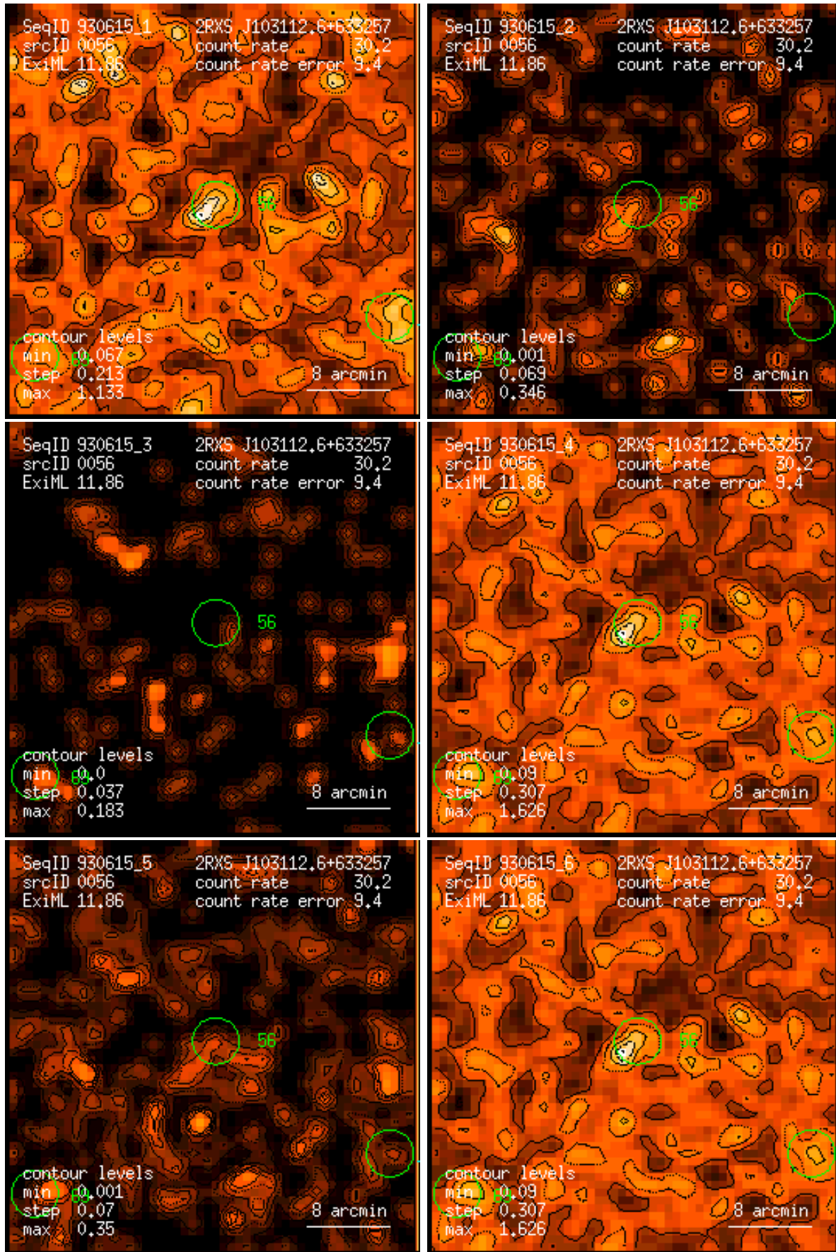
Figure 56: RASS 930615: detection 0056: band rate images, Gaussian filter: (1) PSPC channels 11 – 41, (2) 52 – 90, (3) 91 – 201, (4) 11 – 235, (5) 52 – 201, (6) 11 – 201. Broad band rates in counts/ks. Band rate contour levels in counts/ks/arcmin 2 .
