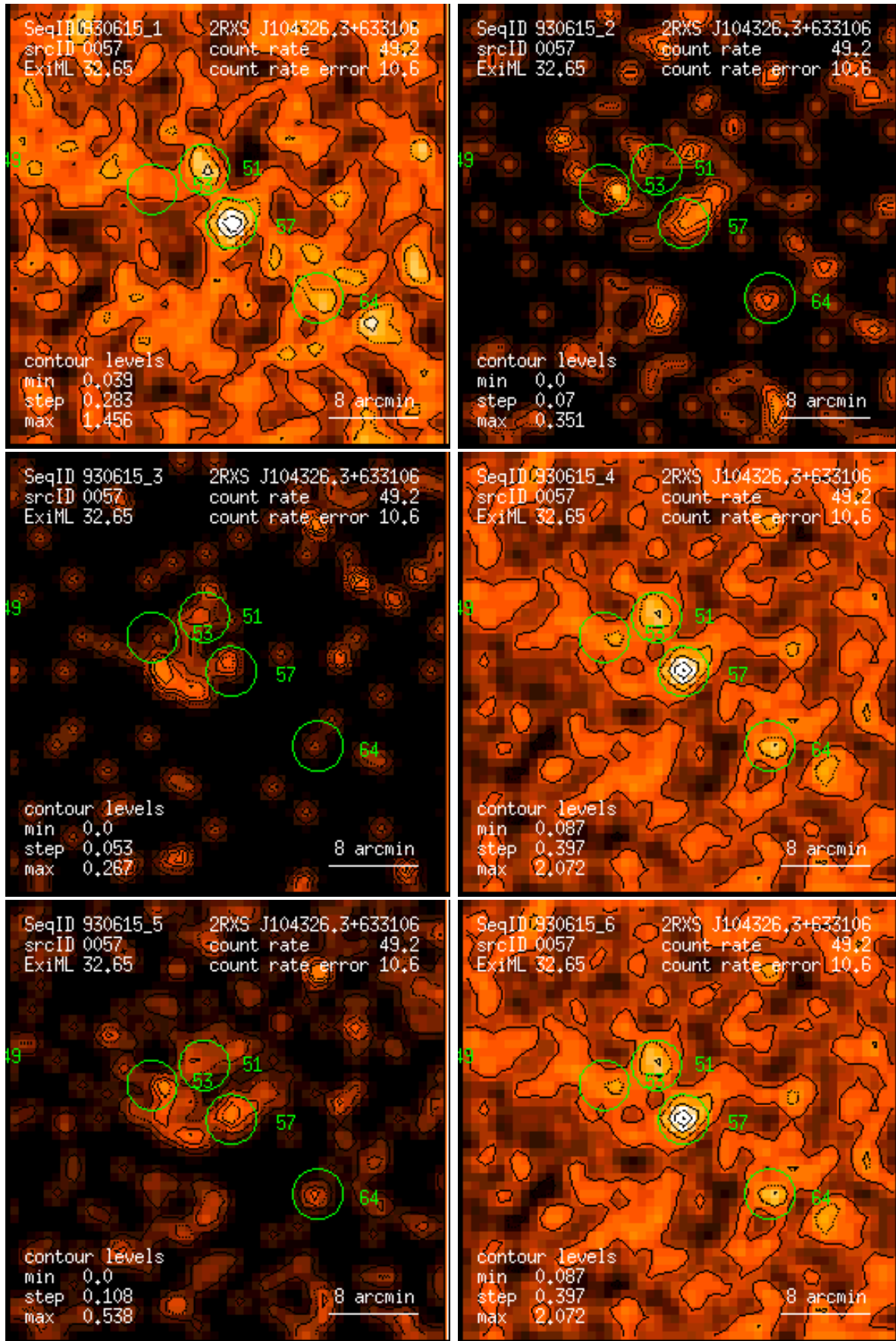
Figure 57: RASS 930615: detection 0057: band rate images, Gaussian filter: (1) PSPC channels 11 – 41, (2) 52 – 90, (3) 91 – 201, (4) 11 – 235, (5) 52 – 201, (6) 11 – 201. Broad band rates in counts/ks. Band rate contour levels in counts/ks/arcmin 2 .
