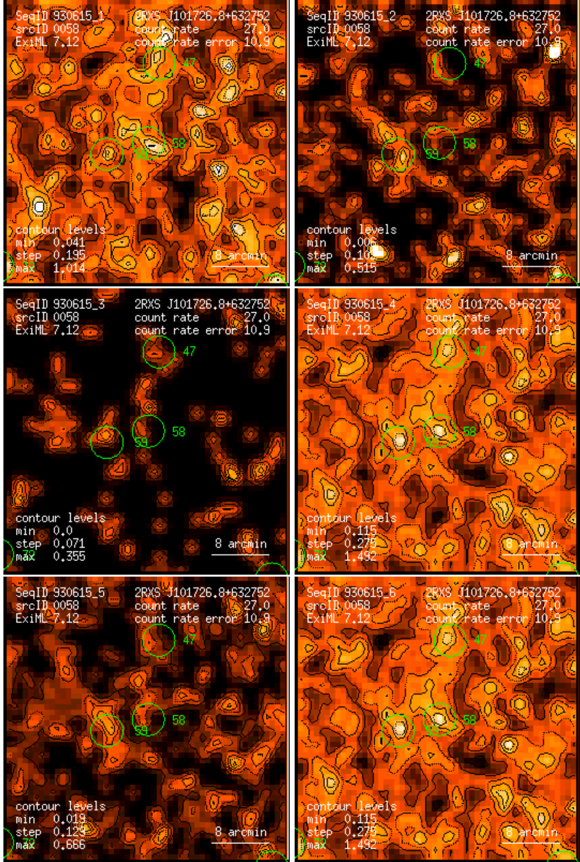
Figure 58: RASS 930615: detection 0058: band rate images, Gaussian filter: (1) PSPC channels 11 – 41, (2) 52 – 90, (3) 91 – 201, (4) 11 – 235, (5) 52 – 201, (6) 11 – 201. Broad band rates in counts/ks. Band rate contour levels in counts/ks/arcmin 2 .
