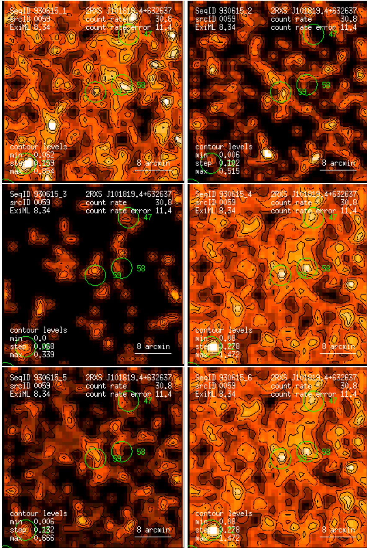
Figure 59: RASS 930615: detection 0059: band rate images, Gaussian filter: (1) PSPC channels 11 – 41, (2) 52 – 90, (3) 91 – 201, (4) 11 – 235, (5) 52 – 201, (6) 11 – 201. Broad band rates in counts/ks. Band rate contour levels in counts/ks/arcmin 2 .
