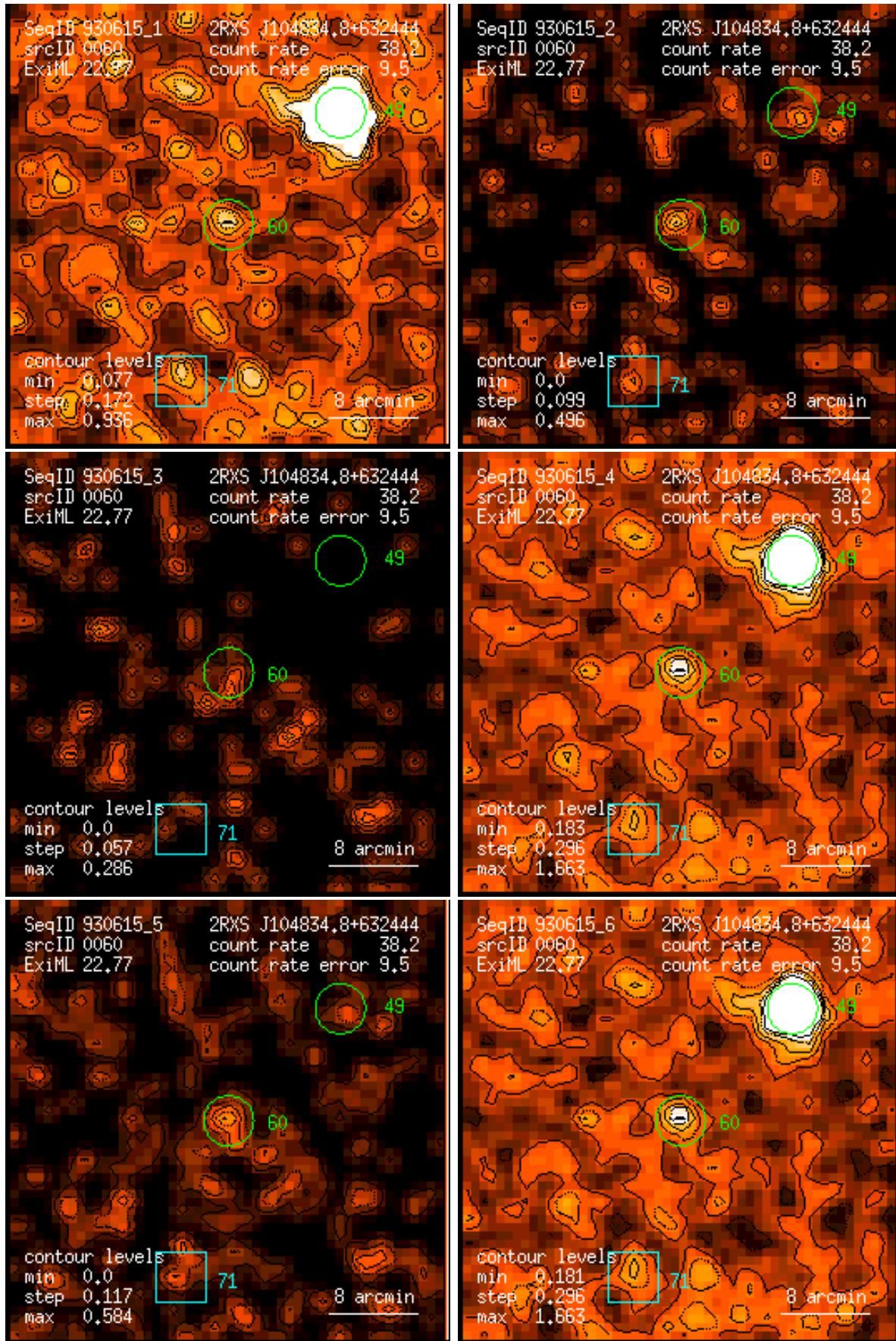
Figure 60: RASS 930615: detection 0060: band rate images, Gaussian filter: (1) PSPC channels 11 – 41, (2) 52 – 90, (3) 91 – 201, (4) 11 – 235, (5) 52 – 201, (6) 11 – 201. Broad band rates in counts/ks. Band rate contour levels in counts/ks/arcmin 2 .
