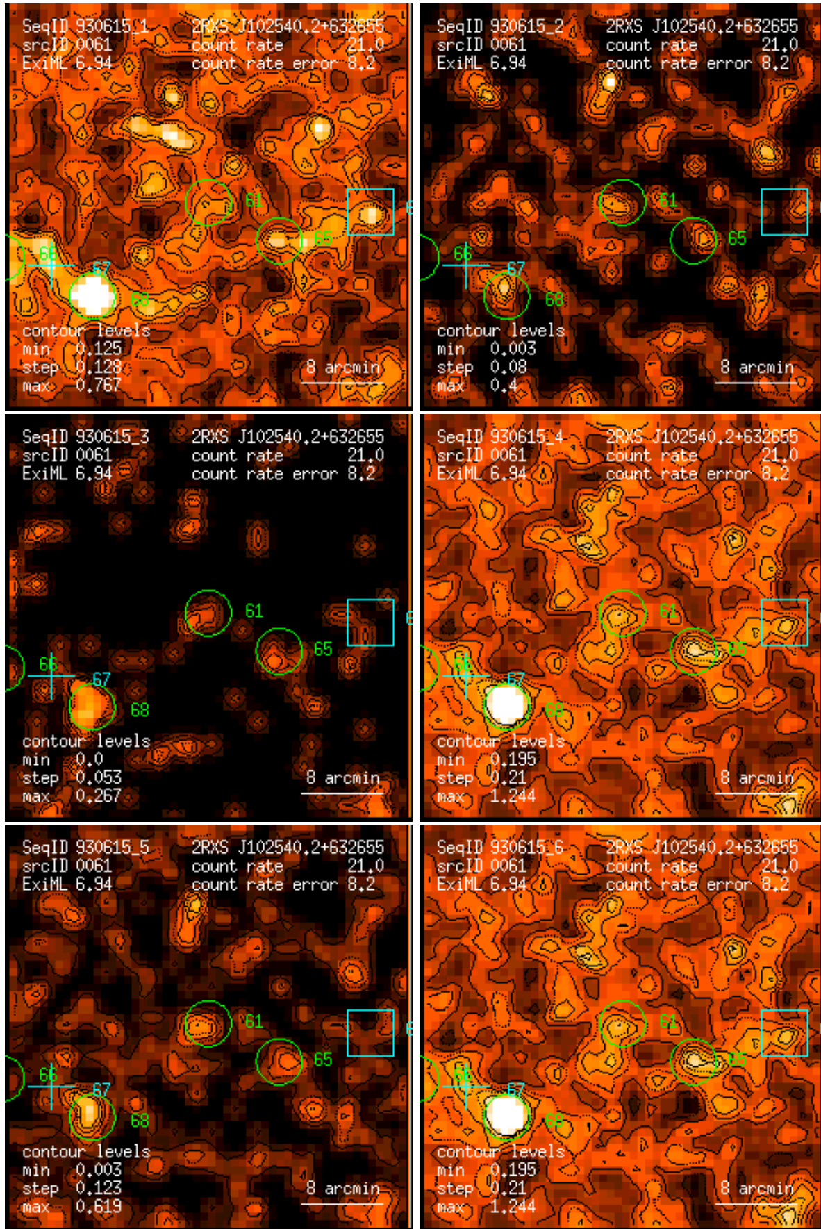
Figure 61: RASS 930615: detection 0061: band rate images, Gaussian filter: (1) PSPC channels 11 – 41, (2) 52 – 90, (3) 91 – 201, (4) 11 – 235, (5) 52 – 201, (6) 11 – 201. Broad band rates in counts/ks. Band rate contour levels in counts/ks/arcmin 2 .
