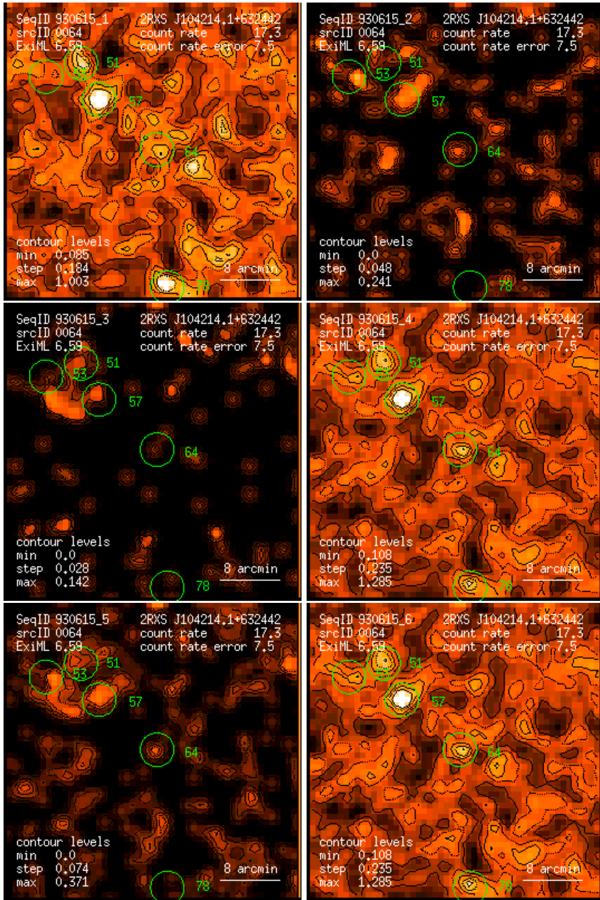
Figure 64: RASS 930615: detection 0064: band rate images, Gaussian filter: (1) PSPC channels 11 – 41, (2) 52 – 90, (3) 91 – 201, (4) 11 – 235, (5) 52 – 201, (6) 11 – 201. Broad band rates in counts/ks. Band rate contour levels in counts/ks/arcmin 2 .
