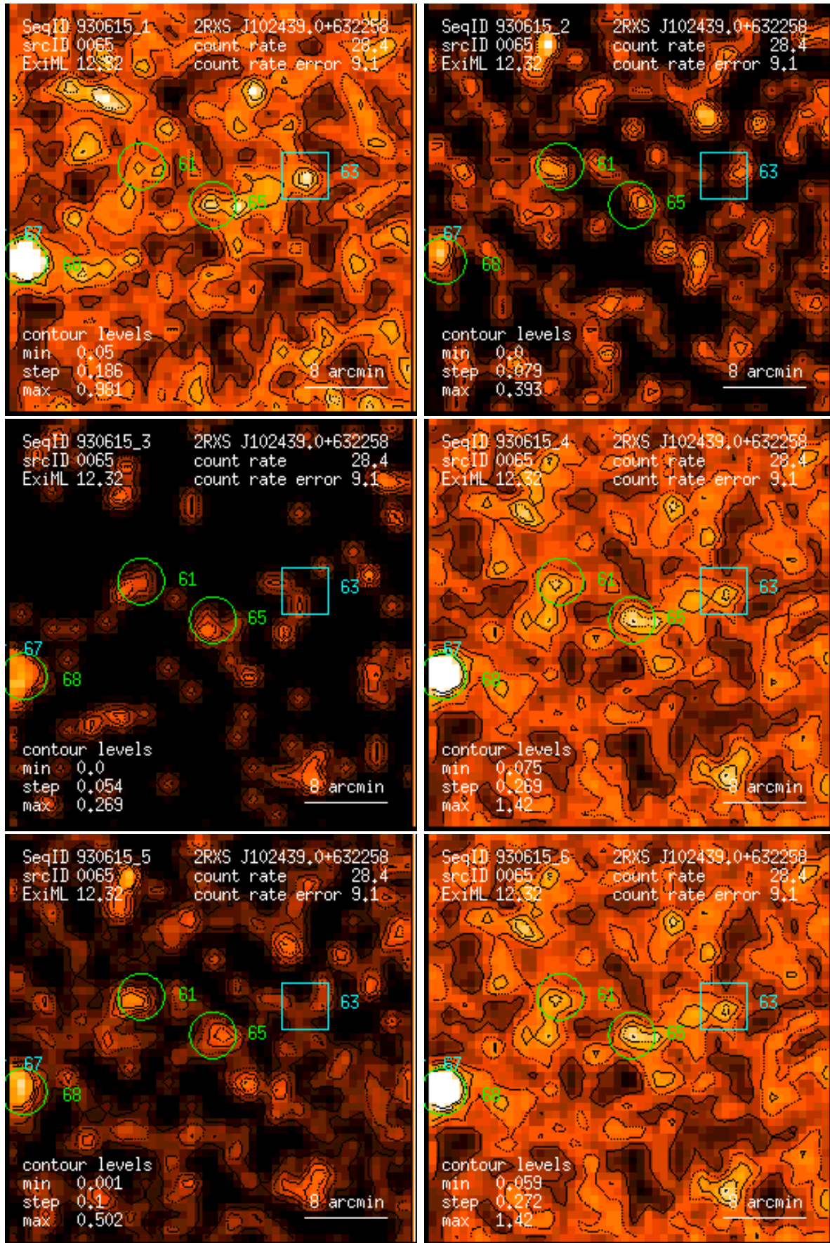
Figure 65: RASS 930615: detection 0065: band rate images, Gaussian filter: (1) PSPC channels 11 – 41, (2) 52 – 90, (3) 91 – 201, (4) 11 – 235, (5) 52 – 201, (6) 11 – 201. Broad band rates in counts/ks. Band rate contour levels in counts/ks/arcmin 2 .
