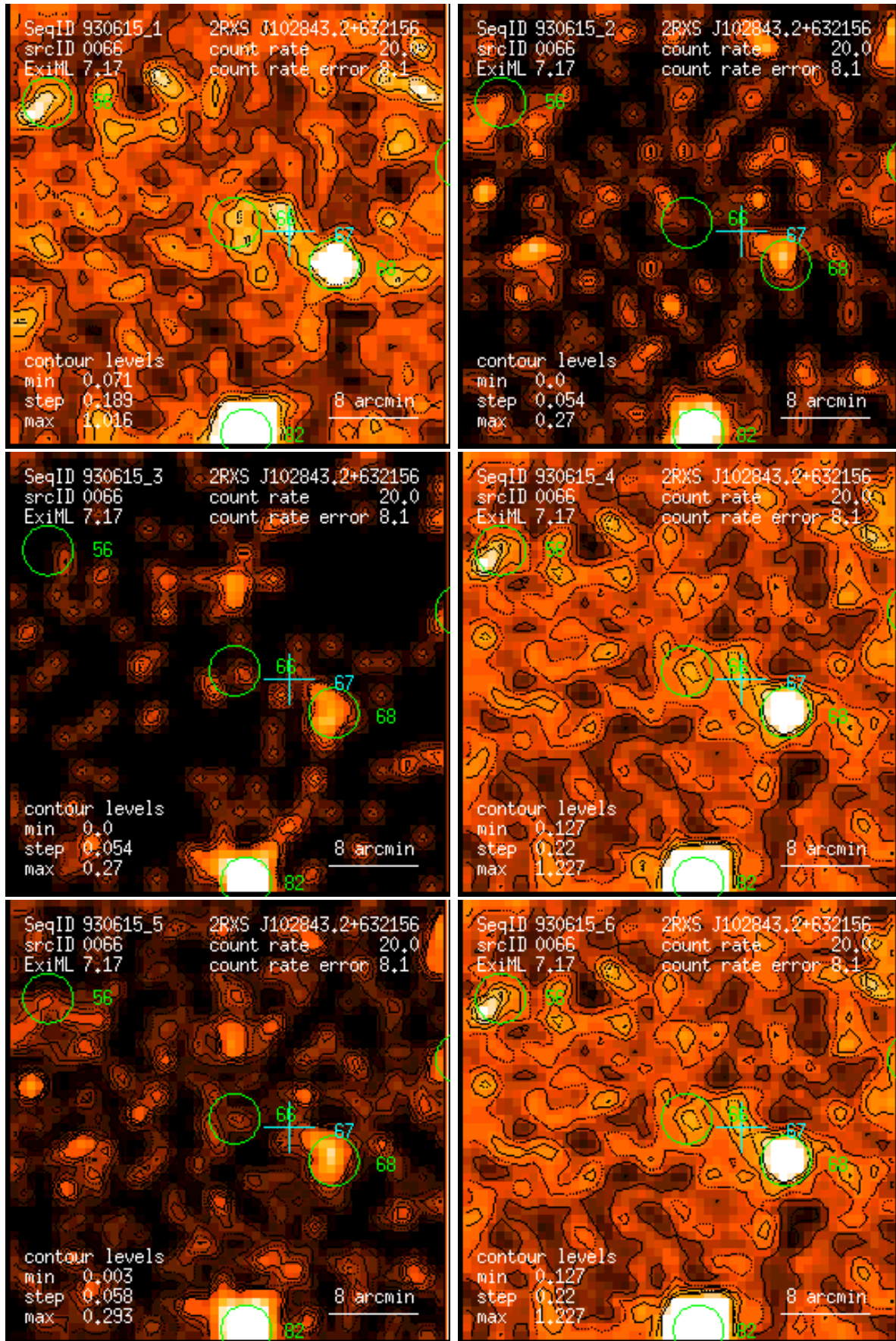
Figure 66: RASS 930615: detection 0066: band rate images, Gaussian filter: (1) PSPC channels 11 – 41, (2) 52 – 90, (3) 91 – 201, (4) 11 – 235, (5) 52 – 201, (6) 11 – 201. Broad band rates in counts/ks. Band rate contour levels in counts/ks/arcmin 2 .
