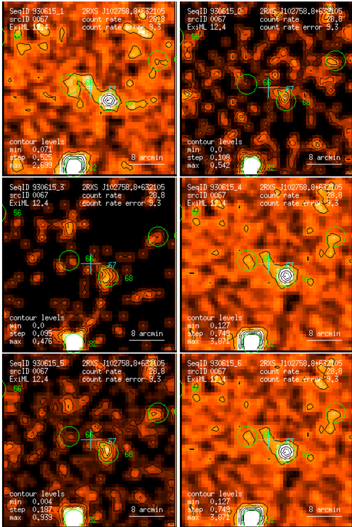
Figure 67: RASS 930615: detection 0067: band rate images, Gaussian filter: (1) PSPC channels 11 – 41, (2) 52 – 90, (3) 91 – 201, (4) 11 – 235, (5) 52 – 201, (6) 11 – 201. Broad band rates in counts/ks. Band rate contour levels in counts/ks/arcmin 2 .
