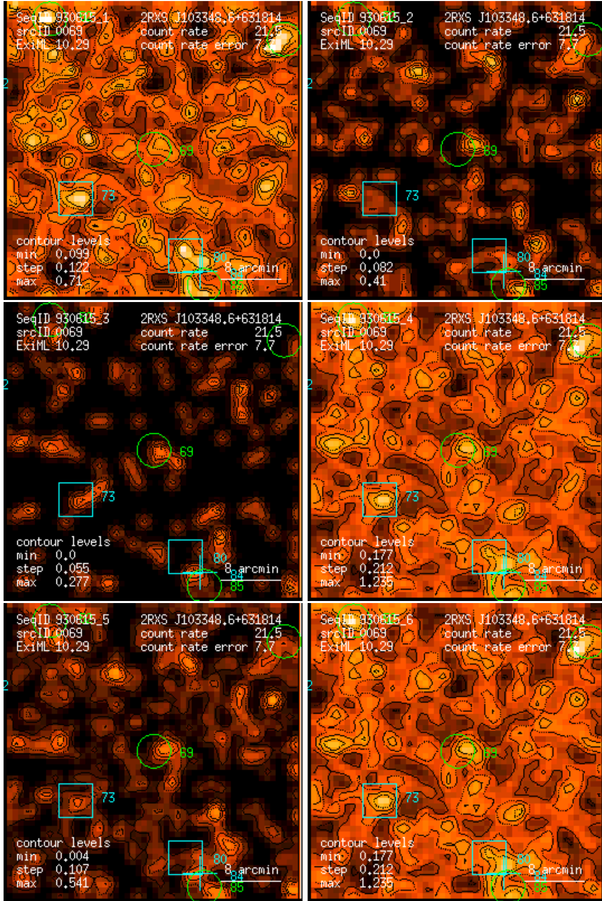
Figure 69: RASS 930615: detection 0069: band rate images, Gaussian filter: (1) PSPC channels 11 – 41, (2) 52 – 90, (3) 91 – 201, (4) 11 – 235, (5) 52 – 201, (6) 11 – 201. Broad band rates in counts/ks. Band rate contour levels in counts/ks/arcmin 2 .
