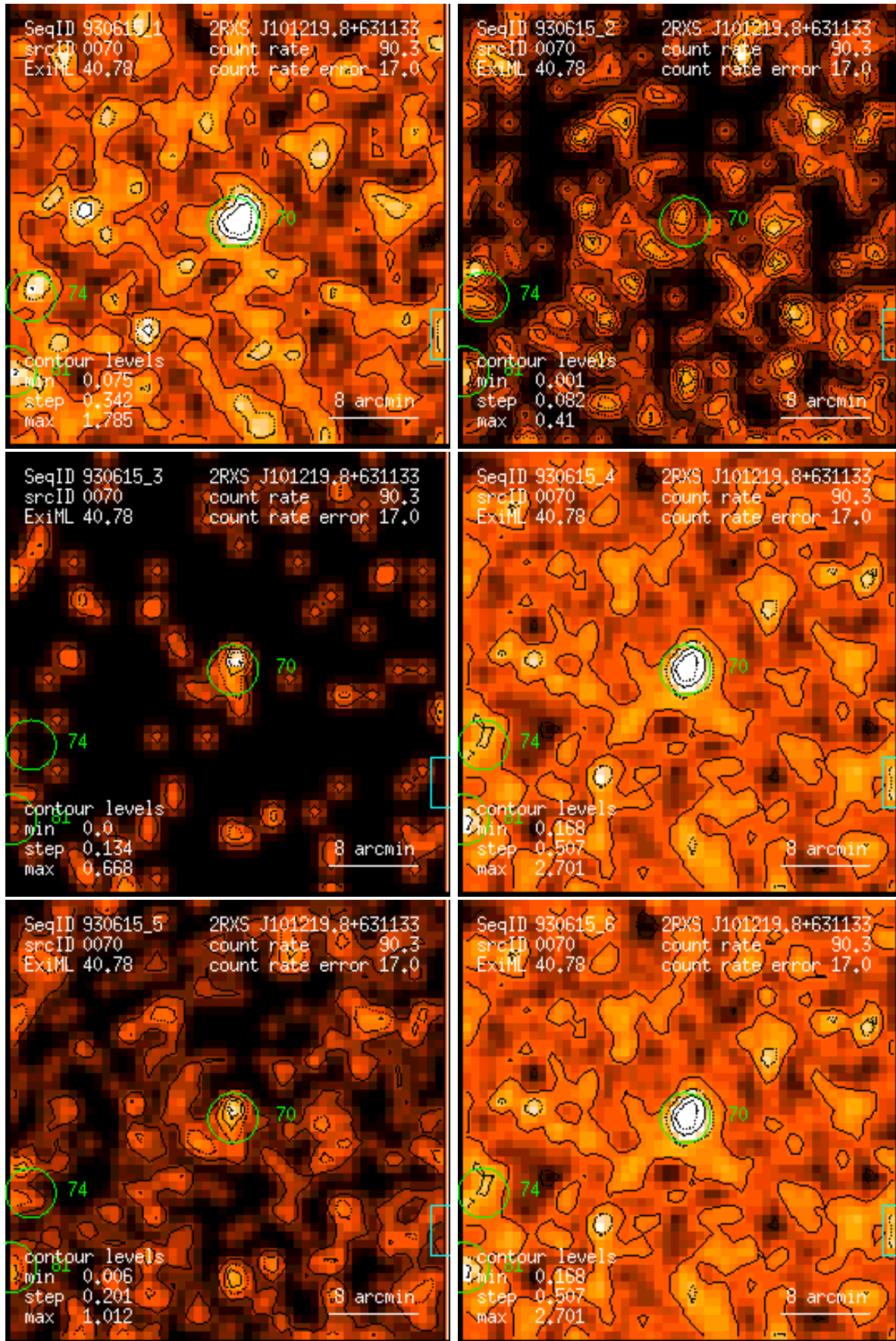
Figure 70: RASS 930615: detection 0070: band rate images, Gaussian filter: (1) PSPC channels 11 – 41, (2) 52 – 90, (3) 91 – 201, (4) 11 – 235, (5) 52 – 201, (6) 11 – 201. Broad band rates in counts/ks. Band rate contour levels in counts/ks/arcmin 2 .
