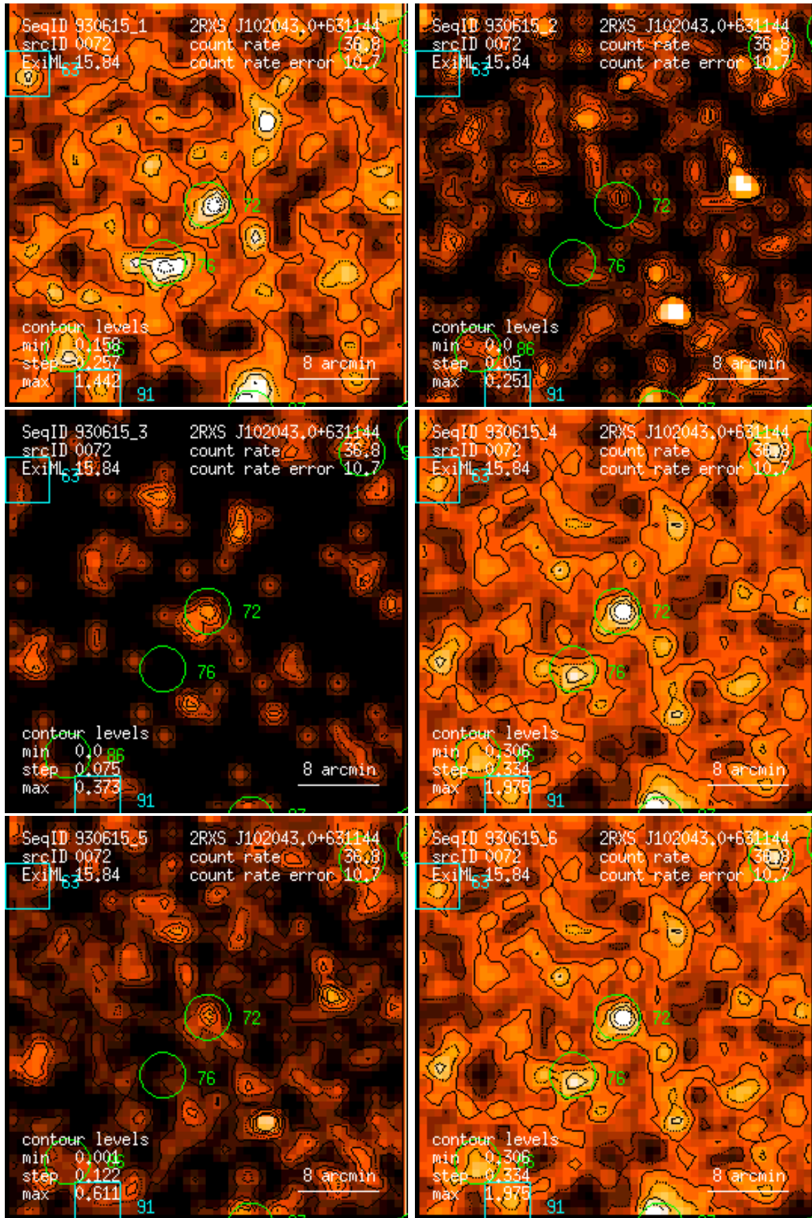
Figure 72: RASS 930615: detection 0072: band rate images, Gaussian filter: (1) PSPC channels 11 – 41, (2) 52 – 90, (3) 91 – 201, (4) 11 – 235, (5) 52 – 201, (6) 11 – 201. Broad band rates in counts/ks. Band rate contour levels in counts/ks/arcmin 2 .
