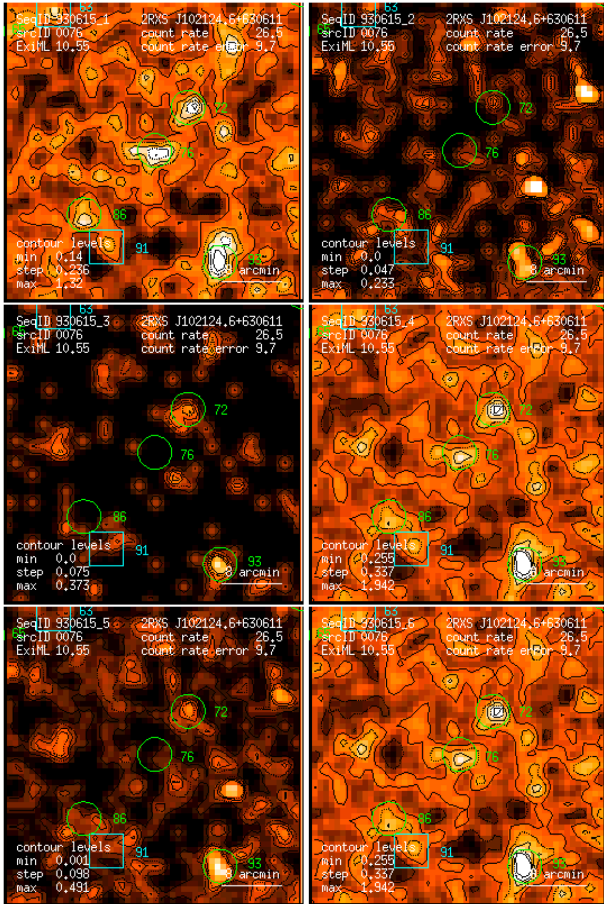
Figure 76: RASS 930615: detection 0076: band rate images, Gaussian filter: (1) PSPC channels 11 – 41, (2) 52 – 90, (3) 91 – 201, (4) 11 – 235, (5) 52 – 201, (6) 11 – 201. Broad band rates in counts/ks. Band rate contour levels in counts/ks/arcmin 2 .
