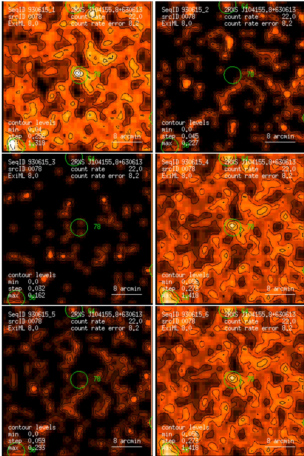
Figure 78: RASS 930615: detection 0078: band rate images, Gaussian filter: (1) PSPC channels 11 – 41, (2) 52 – 90, (3) 91 – 201, (4) 11 – 235, (5) 52 – 201, (6) 11 – 201. Broad band rates in counts/ks. Band rate contour levels in counts/ks/arcmin 2 .
