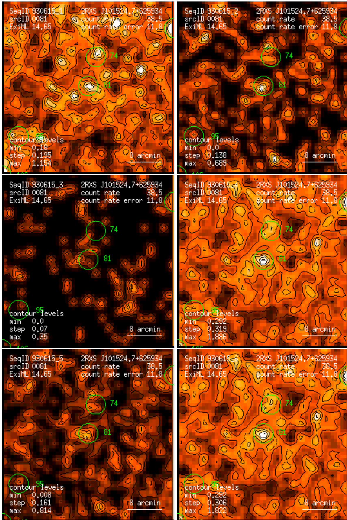
Figure 81: RASS 930615: detection 0081: band rate images, Gaussian filter: (1) PSPC channels 11 – 41, (2) 52 – 90, (3) 91 – 201, (4) 11 – 235, (5) 52 – 201, (6) 11 – 201. Broad band rates in counts/ks. Band rate contour levels in counts/ks/arcmin 2 .
