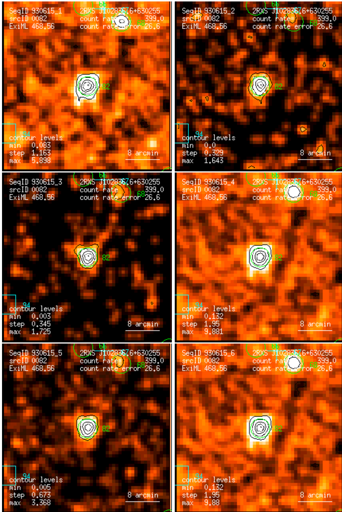
Figure 82: RASS 930615: detection 0082: band rate images, Gaussian filter: (1) PSPC channels 11 – 41, (2) 52 – 90, (3) 91 – 201, (4) 11 – 235, (5) 52 – 201, (6) 11 – 201. Broad band rates in counts/ks. Band rate contour levels in counts/ks/arcmin 2 .
