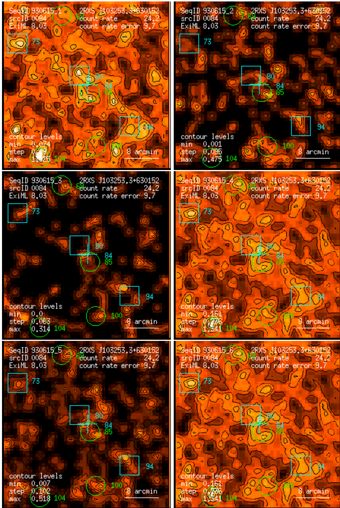
Figure 84: RASS 930615: detection 0084: band rate images, Gaussian filter: (1) PSPC channels 11 – 41, (2) 52 – 90, (3) 91 – 201, (4) 11 – 235, (5) 52 – 201, (6) 11 – 201. Broad band rates in counts/ks. Band rate contour levels in counts/ks/arcmin 2 .
