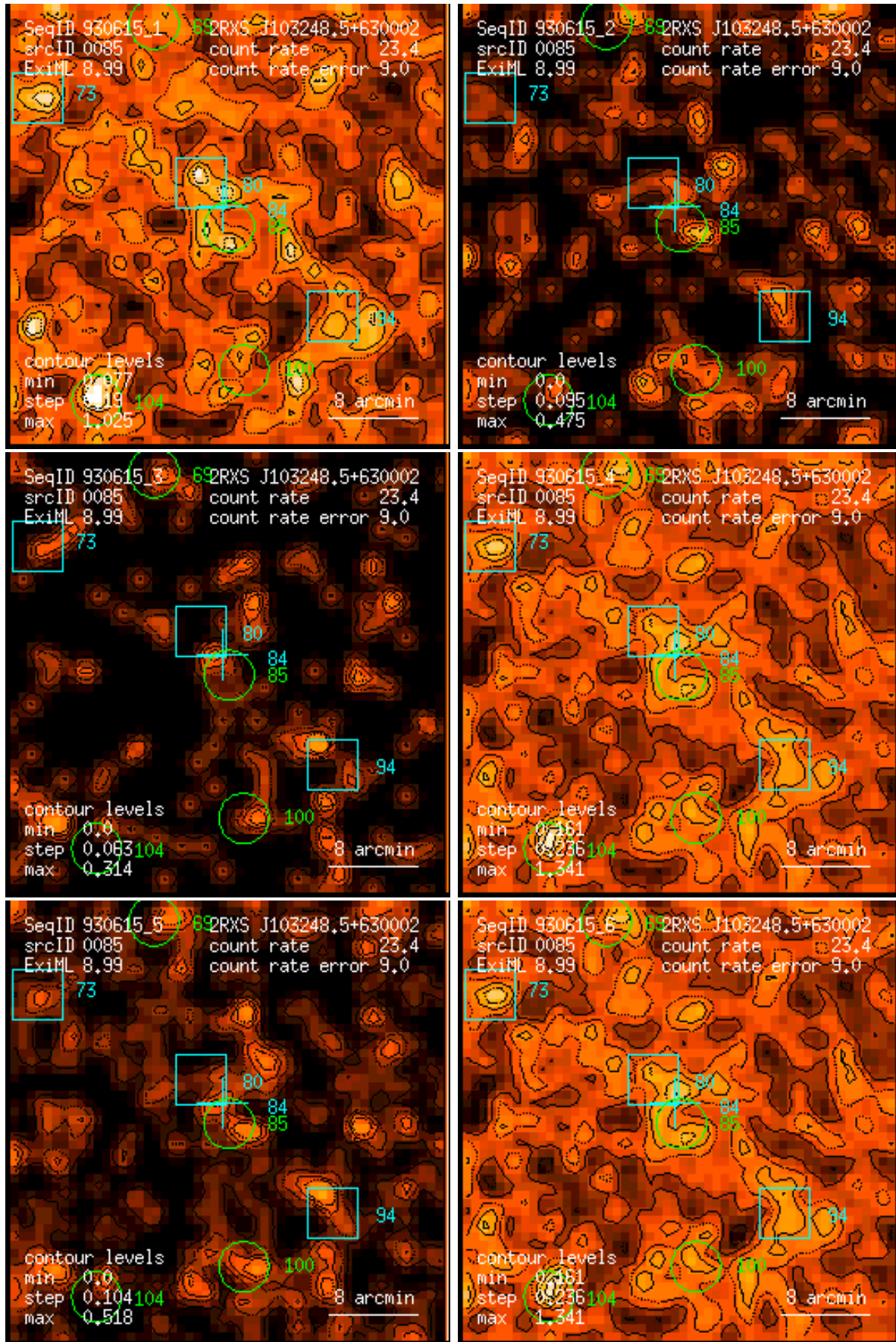
Figure 85: RASS 930615: detection 0085: band rate images, Gaussian filter: (1) PSPC channels 11 – 41, (2) 52 – 90, (3) 91 – 201, (4) 11 – 235, (5) 52 – 201, (6) 11 – 201. Broad band rates in counts/ks. Band rate contour levels in counts/ks/arcmin 2 .
