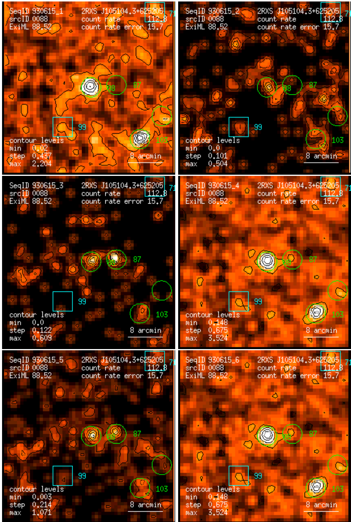
Figure 88: RASS 930615: detection 0088: band rate images, Gaussian filter: (1) PSPC channels 11 – 41, (2) 52 – 90, (3) 91 – 201, (4) 11 – 235, (5) 52 – 201, (6) 11 – 201. Broad band rates in counts/ks. Band rate contour levels in counts/ks/arcmin 2 .
