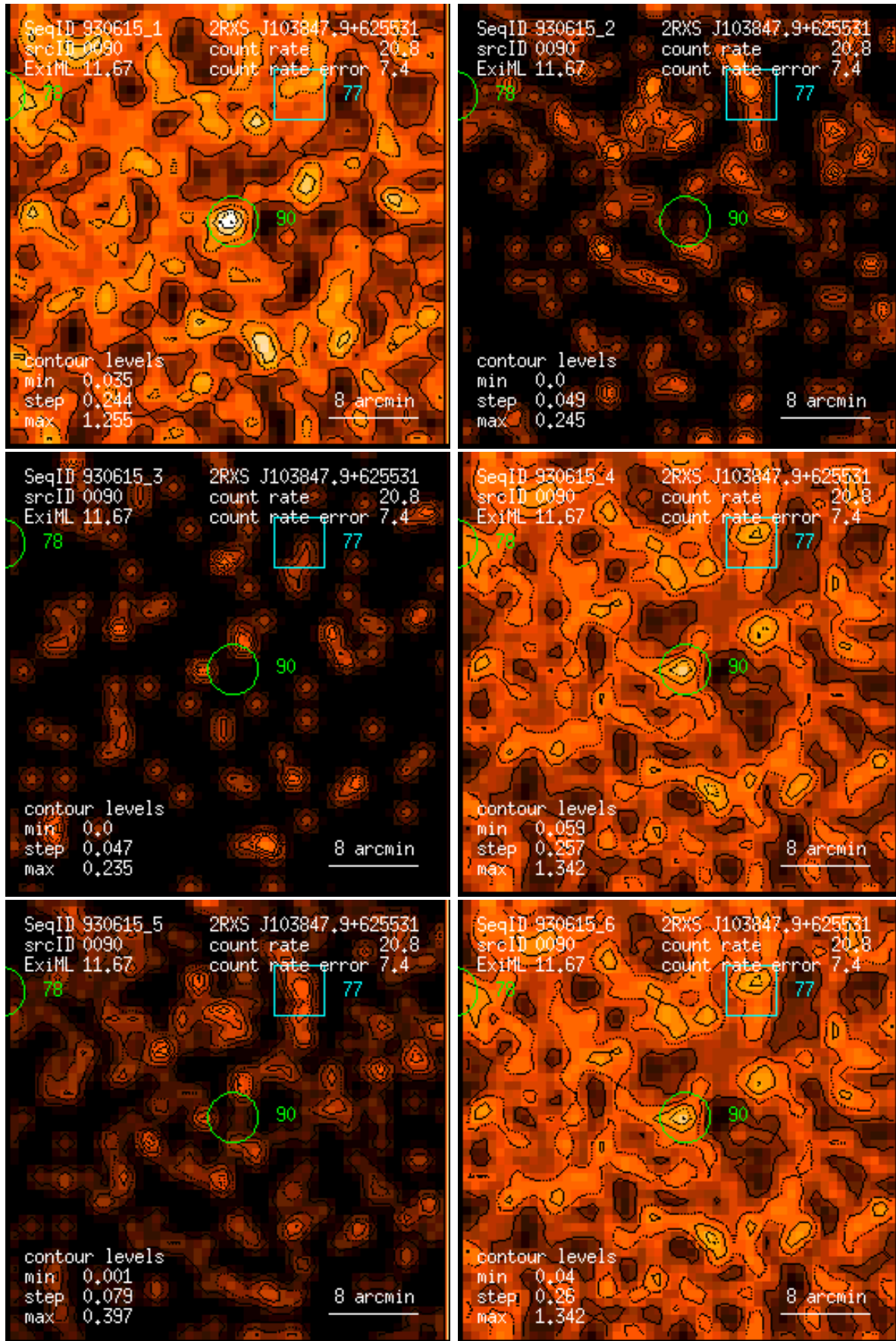
Figure 90: RASS 930615: detection 0090: band rate images, Gaussian filter: (1) PSPC channels 11 – 41, (2) 52 – 90, (3) 91 – 201, (4) 11 – 235, (5) 52 – 201, (6) 11 – 201. Broad band rates in counts/ks. Band rate contour levels in counts/ks/arcmin 2 .
